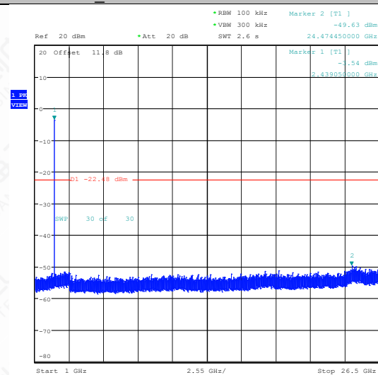
BLE_2M-Ant1-2440-1000~26500-PASS
