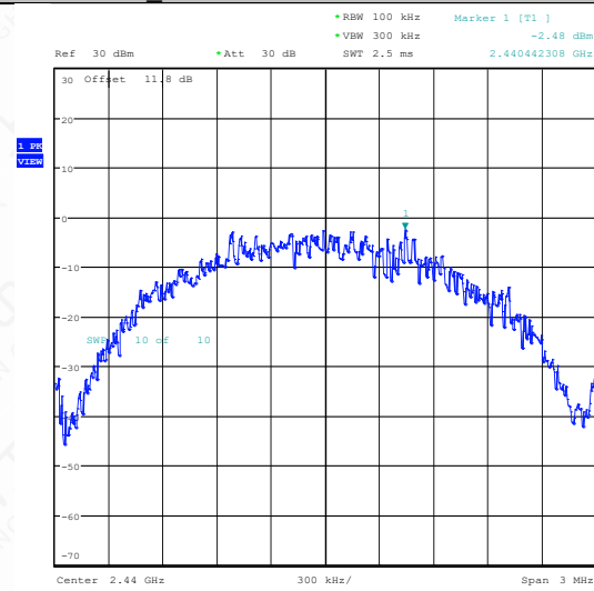
BLE_2M-Ant1-2440-0~Reference-PASS
