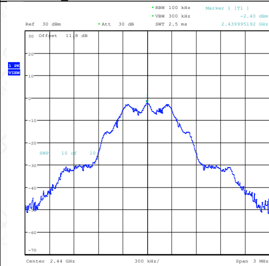
BLE_125K-Ant1-2440-0~Reference-PASS
