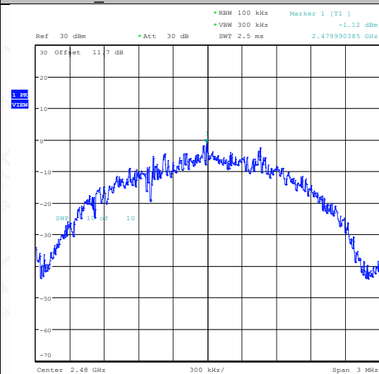
BLE_2M-Ant1-2480-0~Reference-PASS
