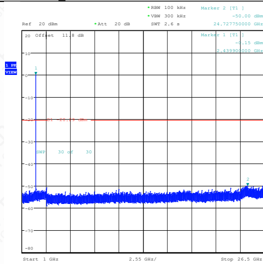
BLE_500K-Ant1-2440-1000~26500-PASS
