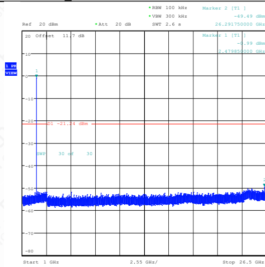
BLE_1M-Ant1-2480-1000~26500-PASS
