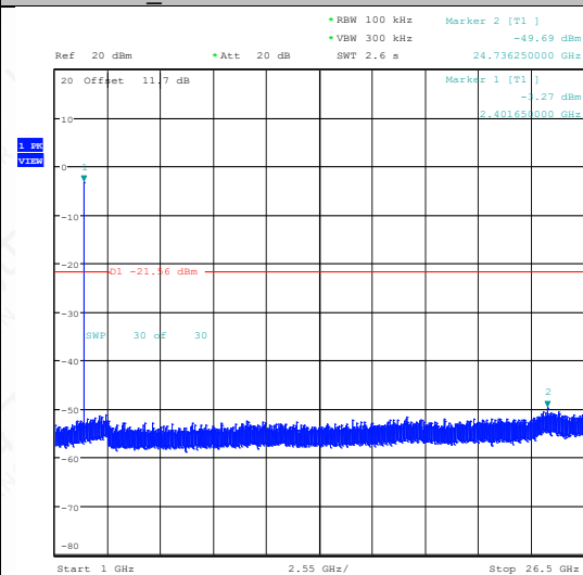
BLE_2M-Ant1-2402-1000~26500-PASS
