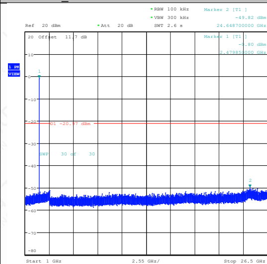
BLE_500K-Ant1-2480-1000~26500-PASS
