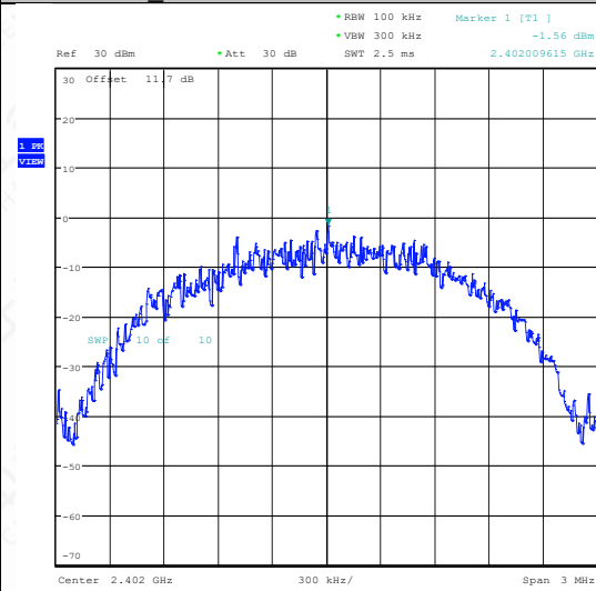
BLE_2M-Ant1-2402-0~Reference-PASS
