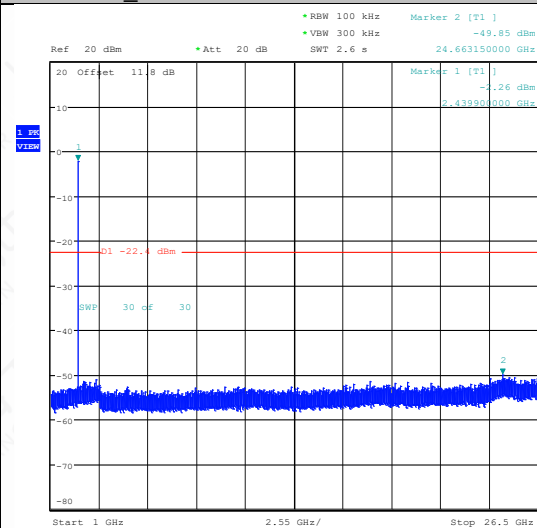
BLE_125K-Ant1-2440-1000~26500-PASS
