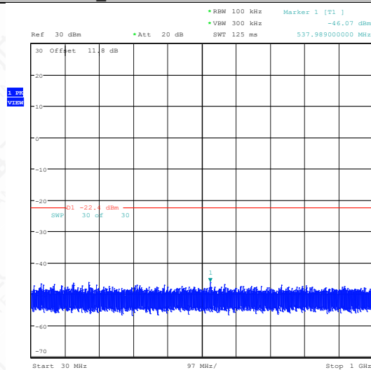
BLE_125K-Ant1-2440-30~1000-PASS
