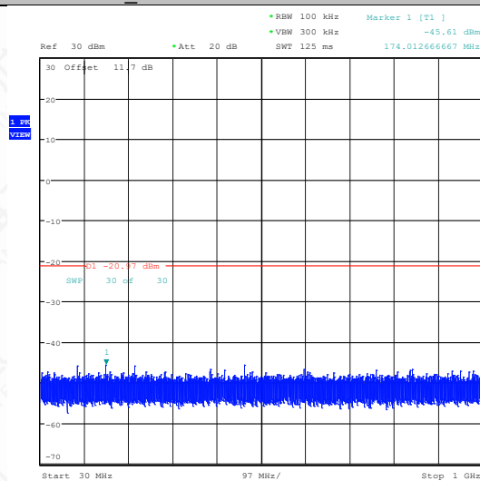
BLE_500K-Ant1-2480-30~1000-PASS
