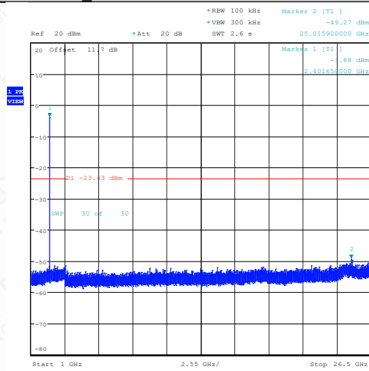
BLE_125K-Ant1-2402-1000~26500-PASS
