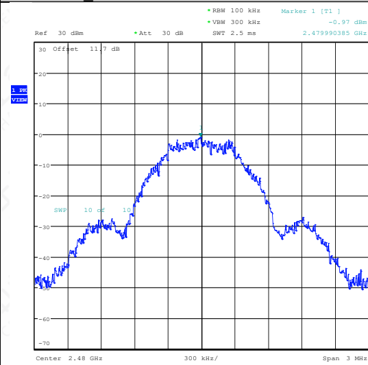
BLE_500K-Ant1-2480-0~Reference-PASS
