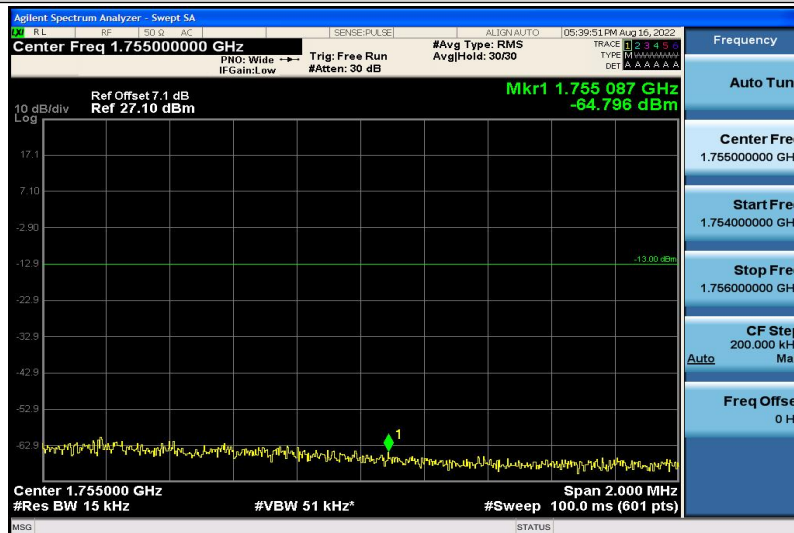
Band4-20MHz-16QAM-20300-1RB#5
