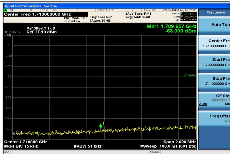
Band4-15MHz-QPSK-20025-1RB#5
