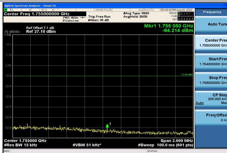
Band4-20MHz-QPSK-20300-1RB#5
