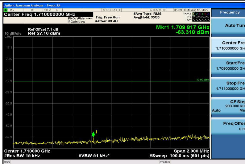
Band4-20MHz-16QAM-20050-1RB#5
