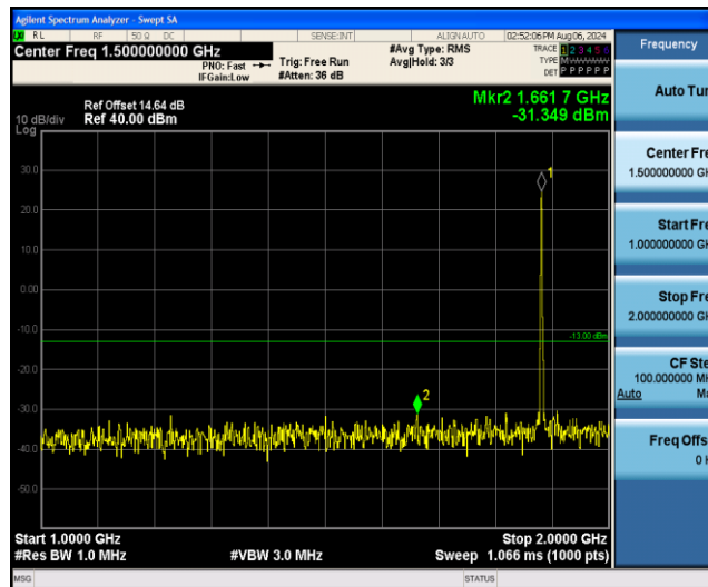
Band2-1.4MHz-16QAM-18900-1RB#0-Range5:2000~20000MHz
