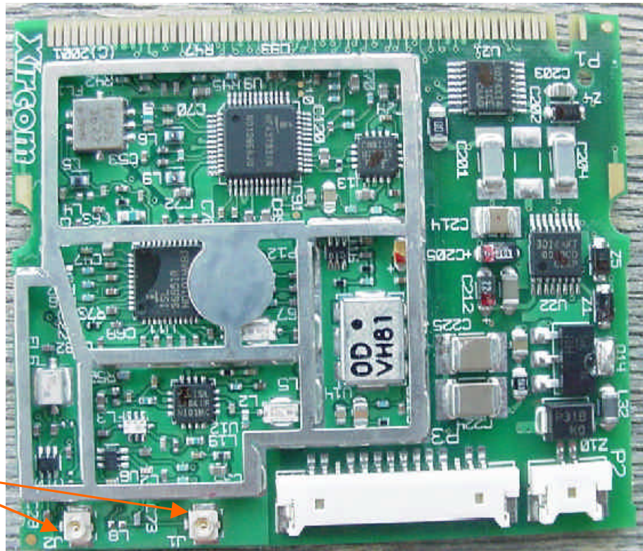
Antenna terminals
