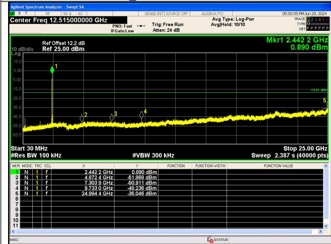
Spurious Emissions IEEE 802.11ax_Channel 6_40MHz_Antenna 0_RU&Index SU
