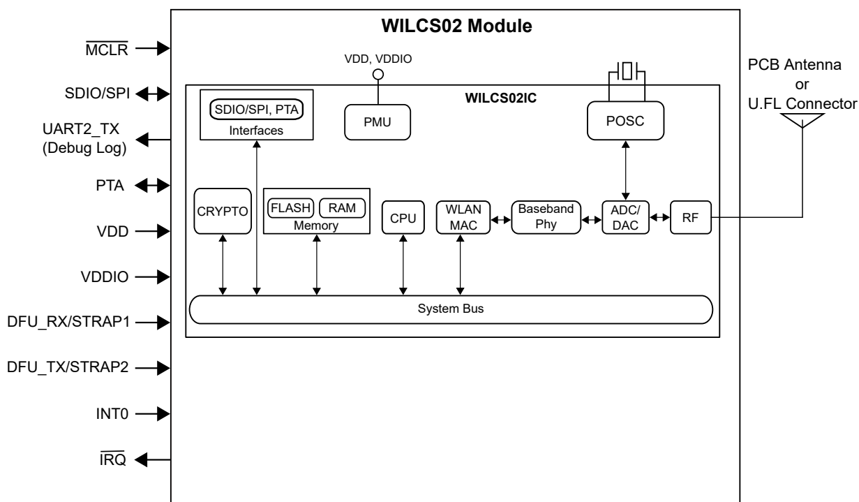
Figure 2-1. WILCS02 Module Block Diagram
