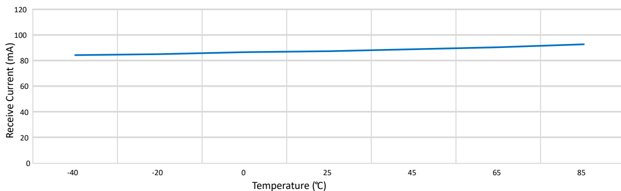
Figure 3-15. Receive Current vs Temperature, MCS7, Channel 7, 3.3V
