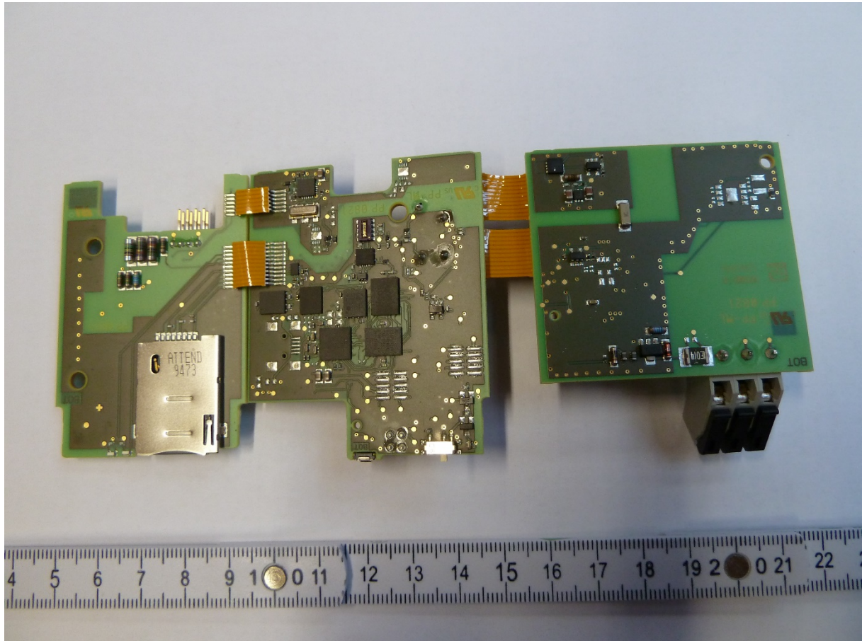
PLICSMOBILE T81 PCB bottom view:
