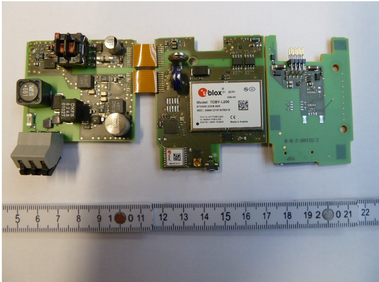
PLICSMOBILE T81 PCB top view:
