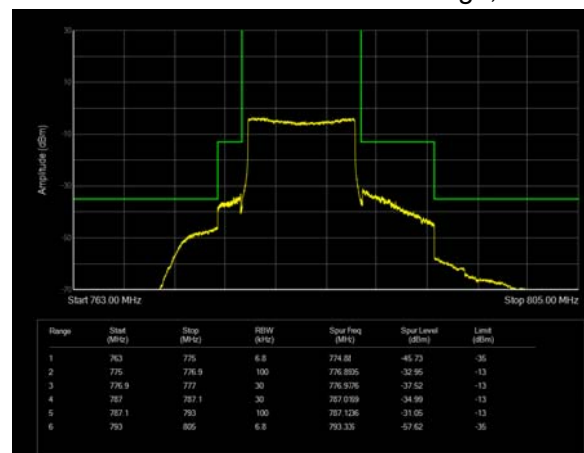
LTE Band 13 64QAM 5MHz CH-High, 1 RB
