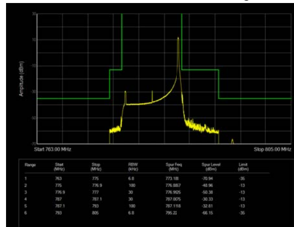
LTE Band 13 16QAM 10MHz CH-High, 100%RB
