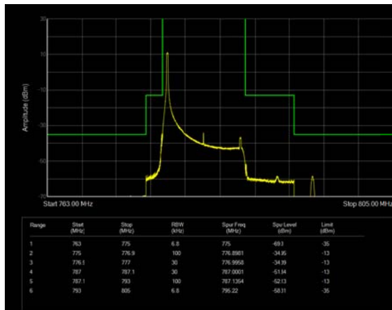
LTE Band 13 16QAM 10MHz CH-Low, 100%RB
