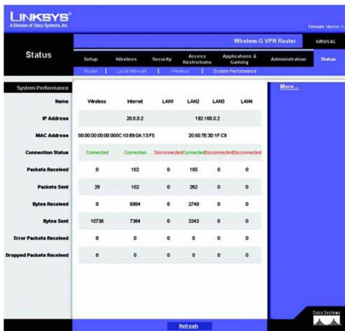
Figure 6-39: System Performance
