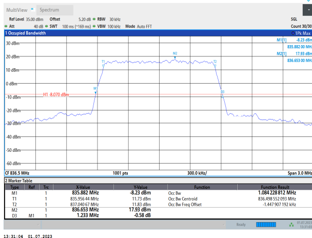
Band5-1.4MHz-QPSK-20525-6RB#0
