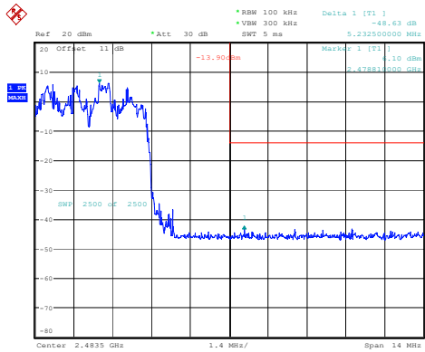
3DH1_Hopping_Upper
