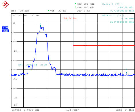
3DH1_High
