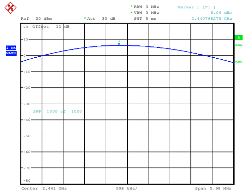
2DH1_Middle 6.06dBm
