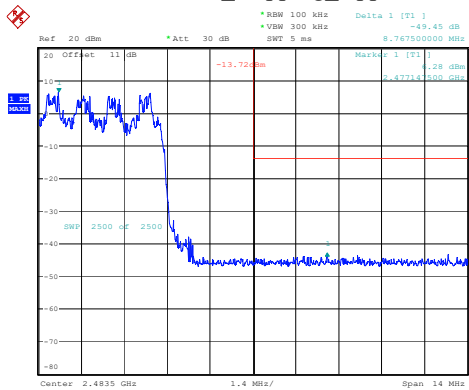
2DH1_Hopping_Upper
