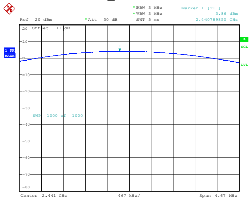
DH1_Middle 3.86dBm
