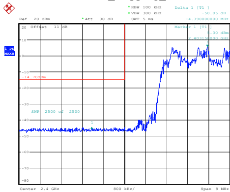
2DH1_Hopping_Lower
