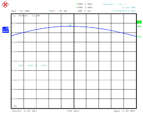
2DH1_High 6.54dBm
