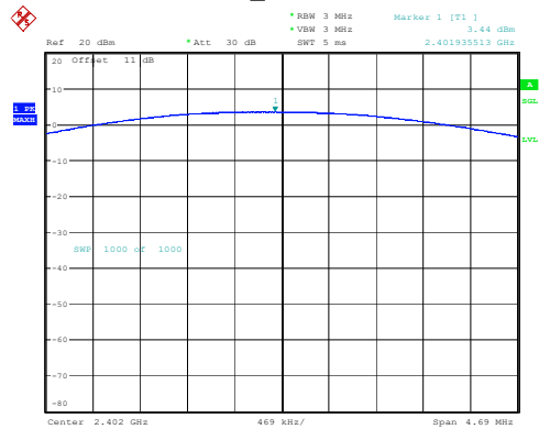
DH1_Low 3.44dBm
