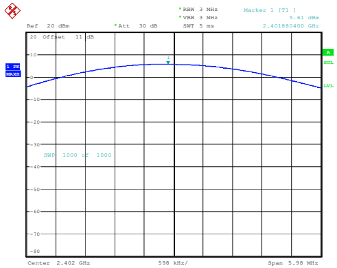
2DH1_Low 5.61dBm
