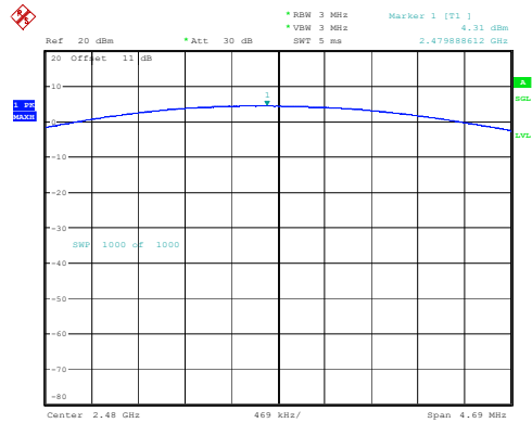
DH1_High 4.31dBm
