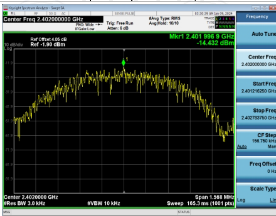
Power_Spectral_Density_NVNT_ANT1_1Mbps_2402
