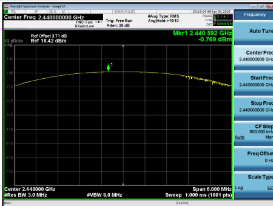
Peak_Output_Power_NVNT_ANT1_1Mbps_2440
