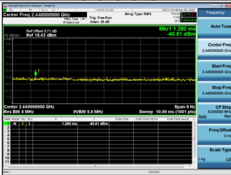
Duty_Cycle_NVNT_ANT1_1Mbps_2440
