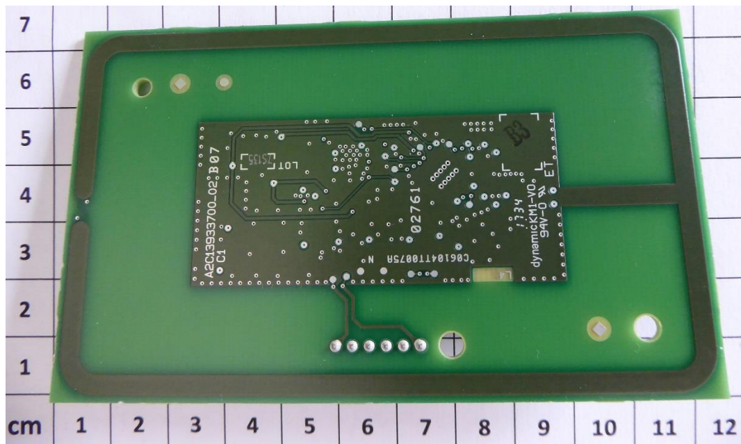
PCB mainboard – bottom view
