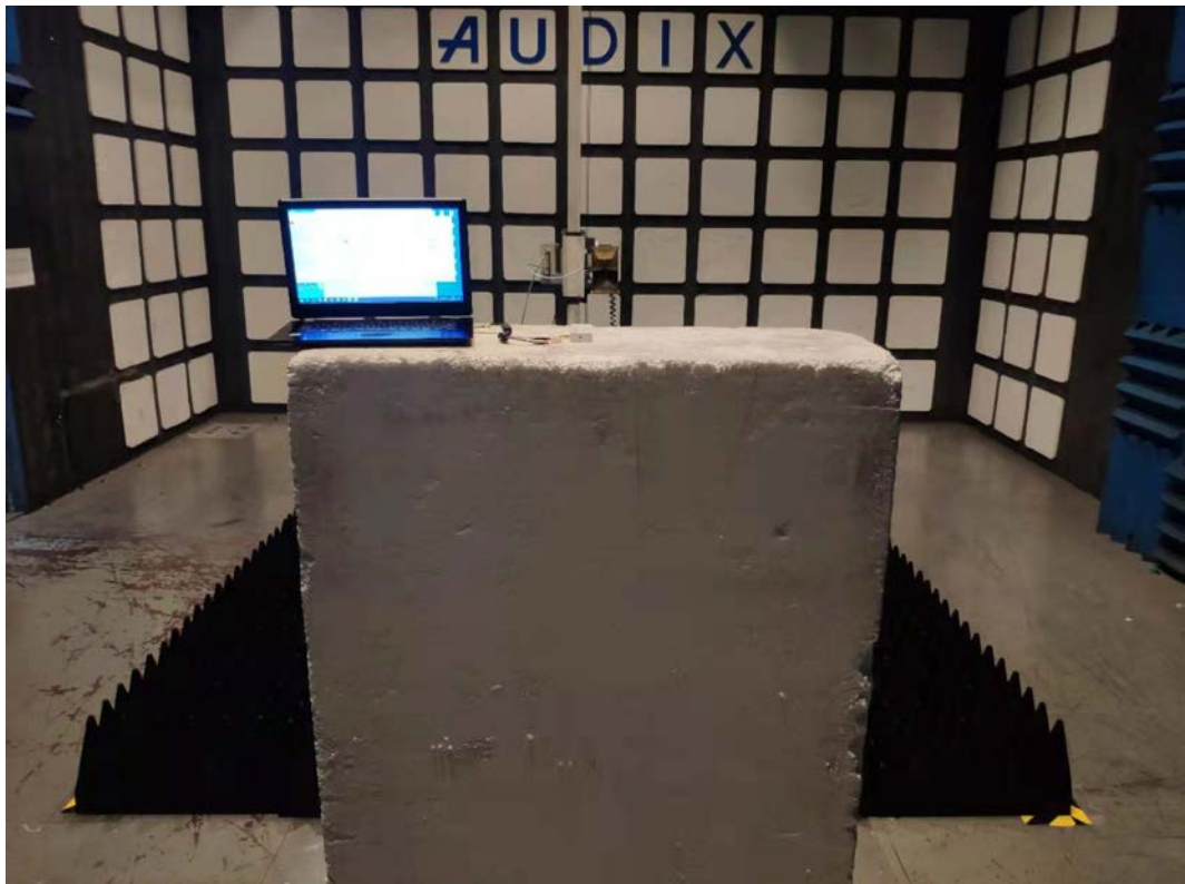
(ABOVE 1GHz)
