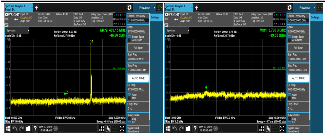
Band17-10MHz-QPSK-23780-1RB#0-Range1:30~1000MHz
