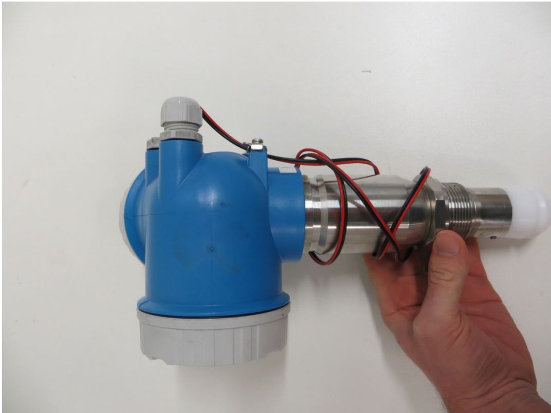
FMR 60 / PTFE Thread 1.5"
