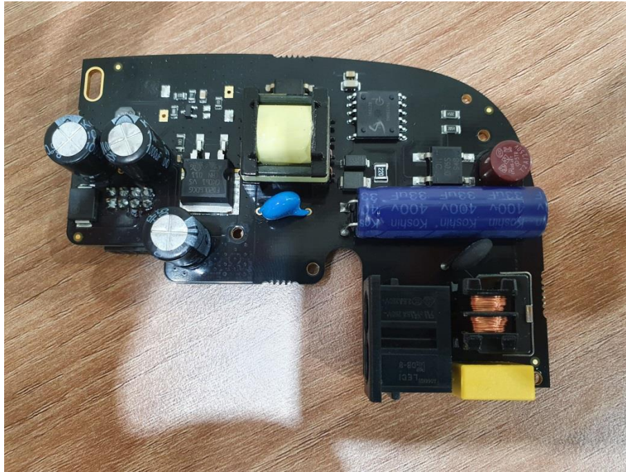
Power Board - Front Top
