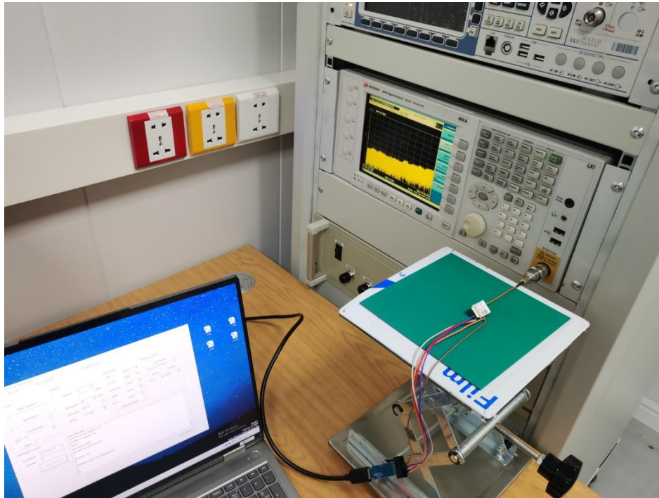
RSE Test Photo(30MHz-1000MHz)
