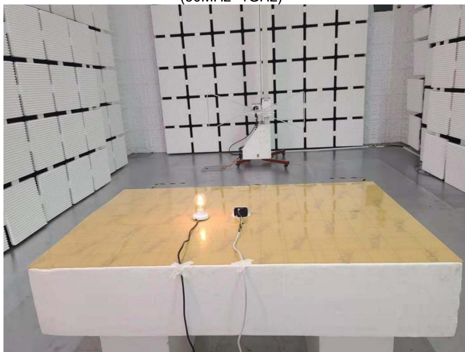
Radiated Emission Test Photo (30MHz- 1GHz)
