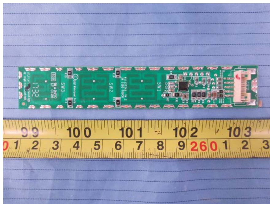
EUT – Switch Board 2 Top View
