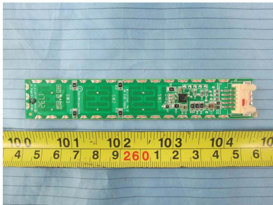
EUT – Switch Board 1 Top View
