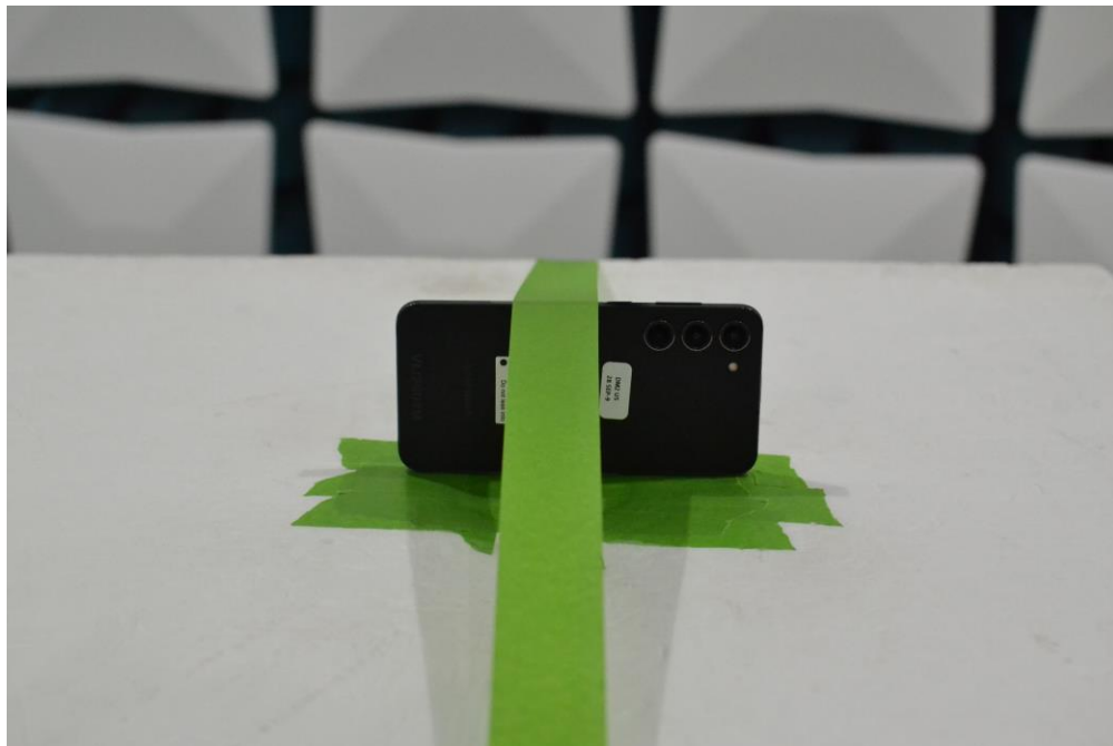
Figure 12. Test Setup – Y Position – 1GHz-18GHz
