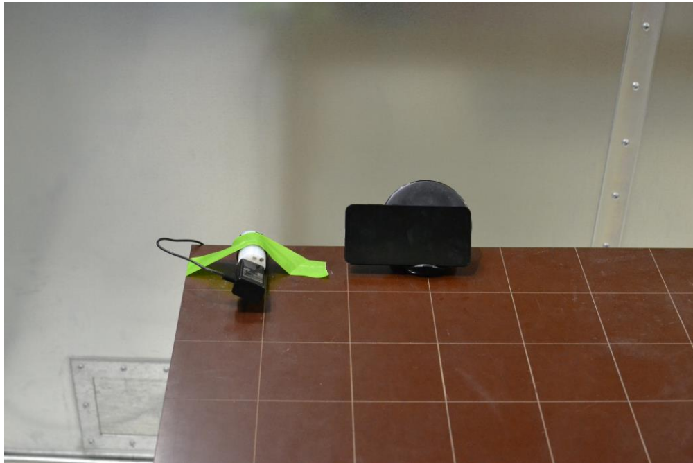
Figure 6. Test Setup – ACLC WCP – <30MHz
