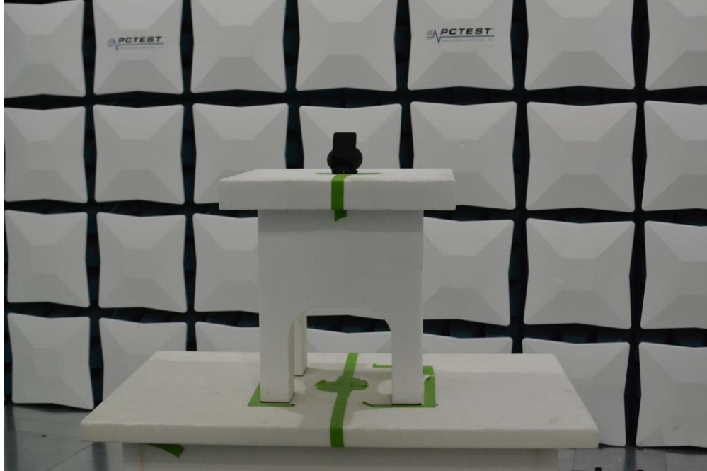
Figure 15. Test Setup – WCP Position – 1GHz-18GHz
