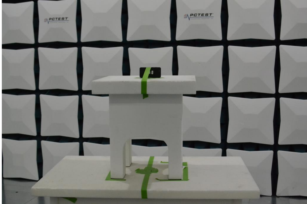
Figure 11. Test Setup – Y Position – 1GHz-18GHz
