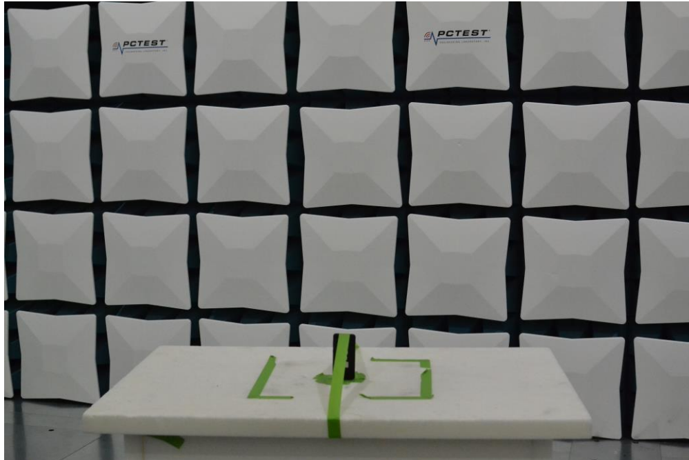
Figure 19. Test Setup – Z Position – 30MHz-1GHz
