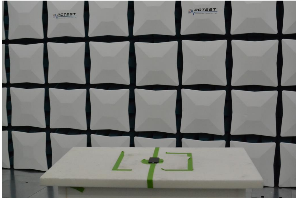
Figure 17. Test Setup – X Position – 30MHz-1GHz
