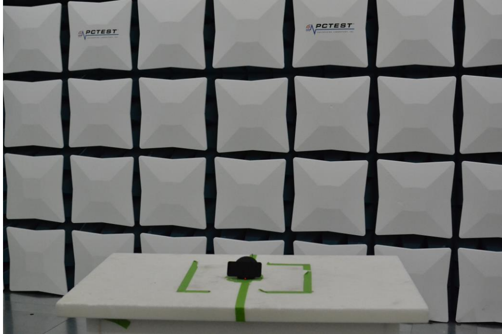
Figure 21. Test Setup – WCP Position – 30MHz-1GHz
