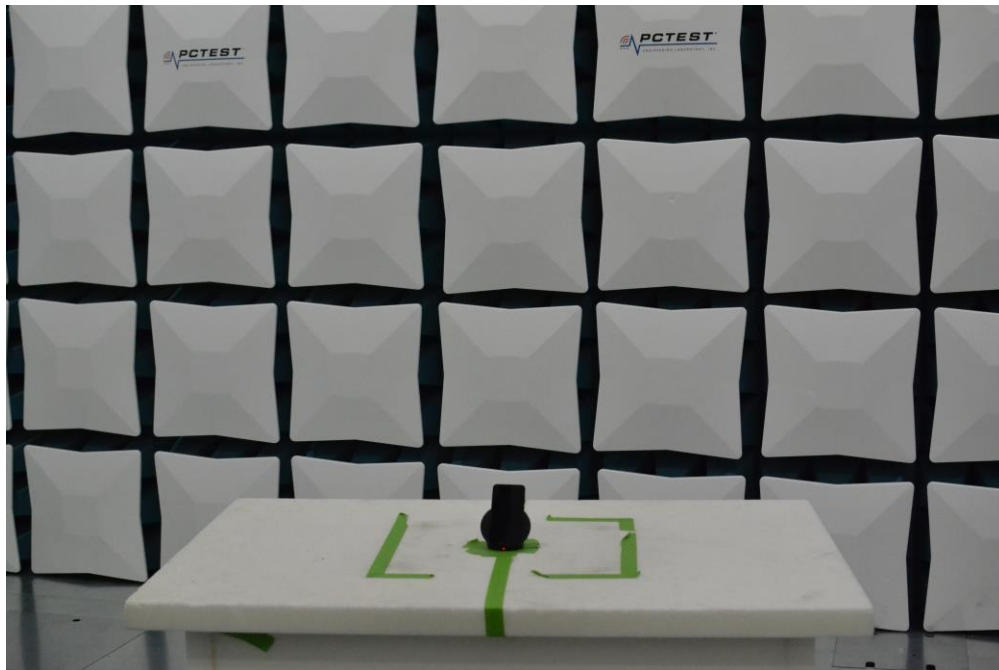
Figure 20. Test Setup – WCP Position – 30MHz-1GHz
