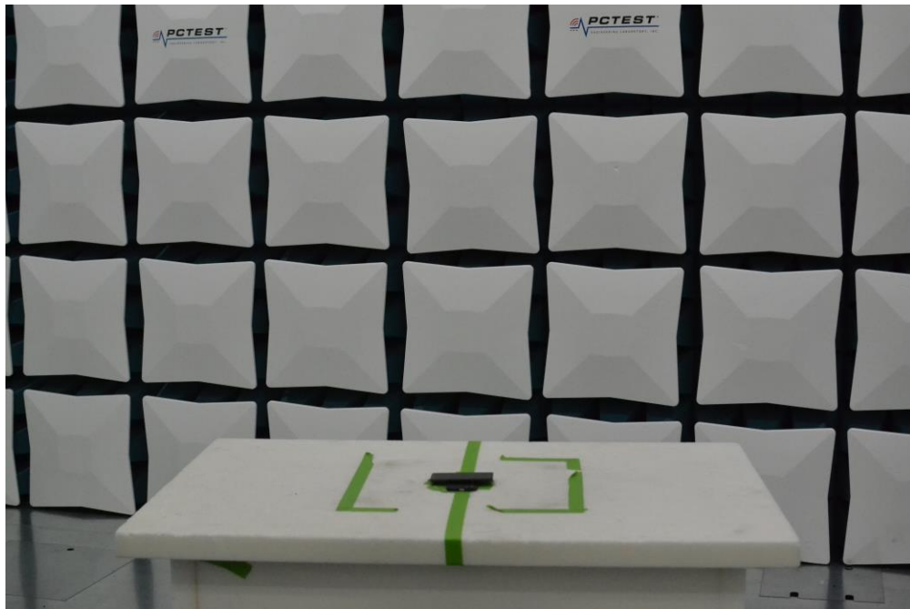
Figure 24. Test Setup – WPT Position – 30Hz-1GHz
