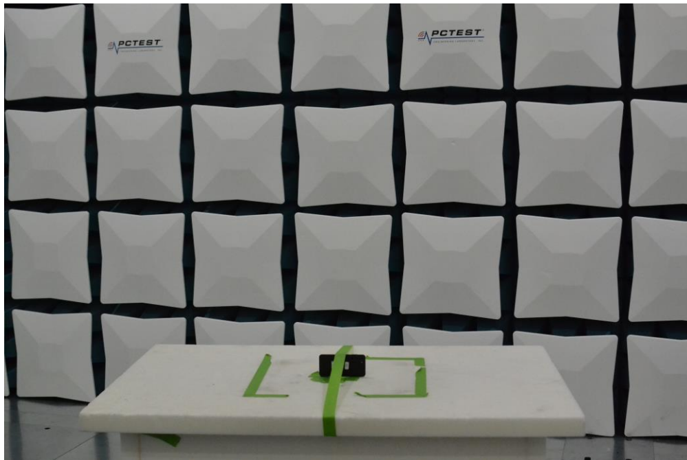
Figure 18. Test Setup – Y Position – 30MHz-1GHz
