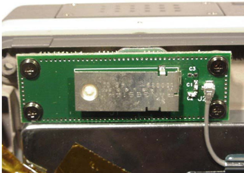
Back of LCD Display - Right-Side Antenna
