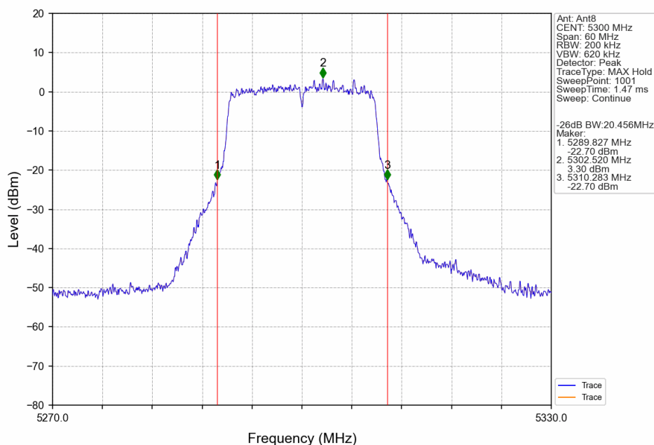
802.11n(HT20)_MCH_5300MHz_Ant8_NTNV
