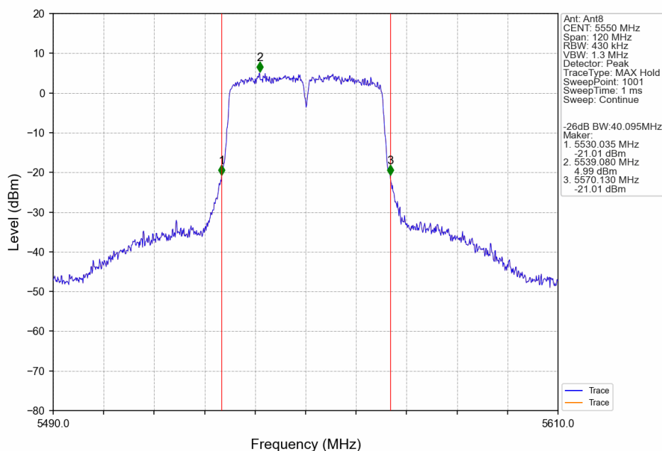
802.11n(HT40)_MCH_5550MHz_Ant8_NTNV
