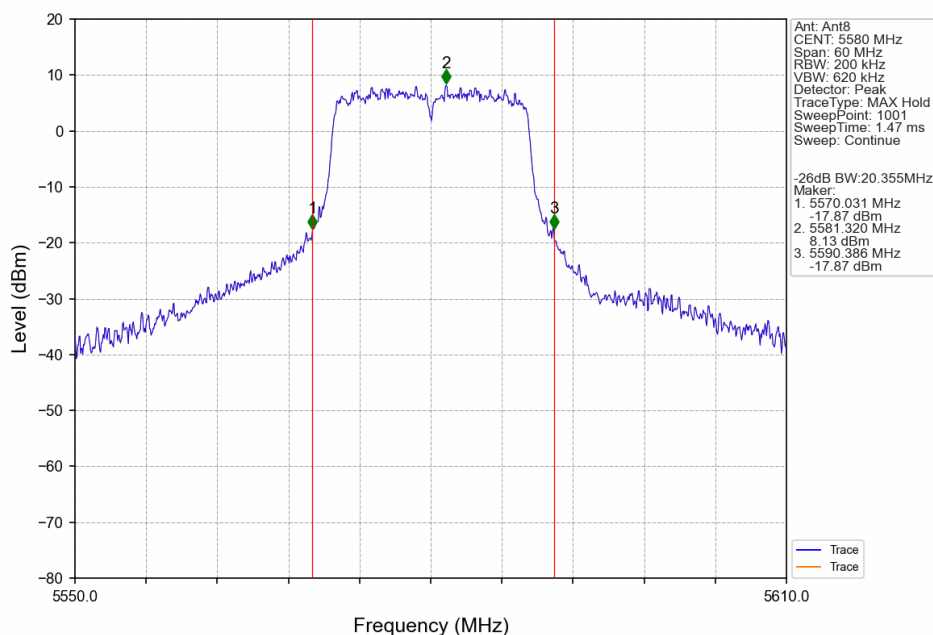
802.11a_MCH_5580MHz_Ant8_NTNV
