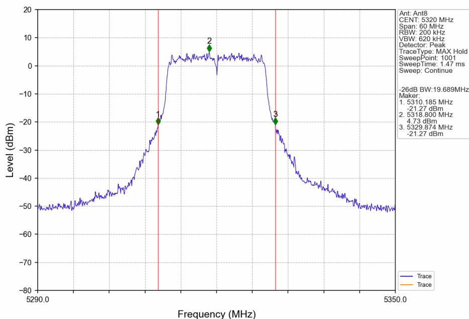
802.11a_HCH_5320MHz_Ant8_NTNV
