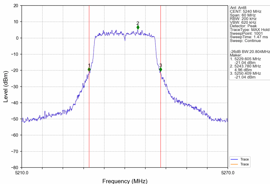
802.11n(HT20)_HCH_5240MHz_Ant8_NTNV
