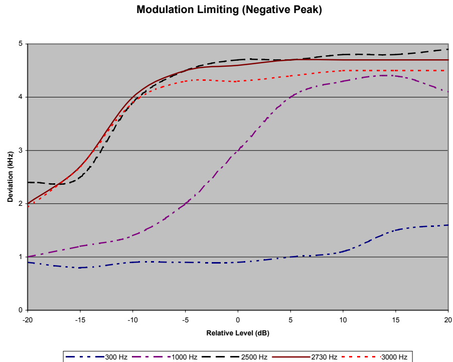
PLOT 8-1: MODULATION LIMITING RESPONSE – 155.0 MHZ {25 KHZ CHANNEL SPACING} NEGATIVE PEAK
