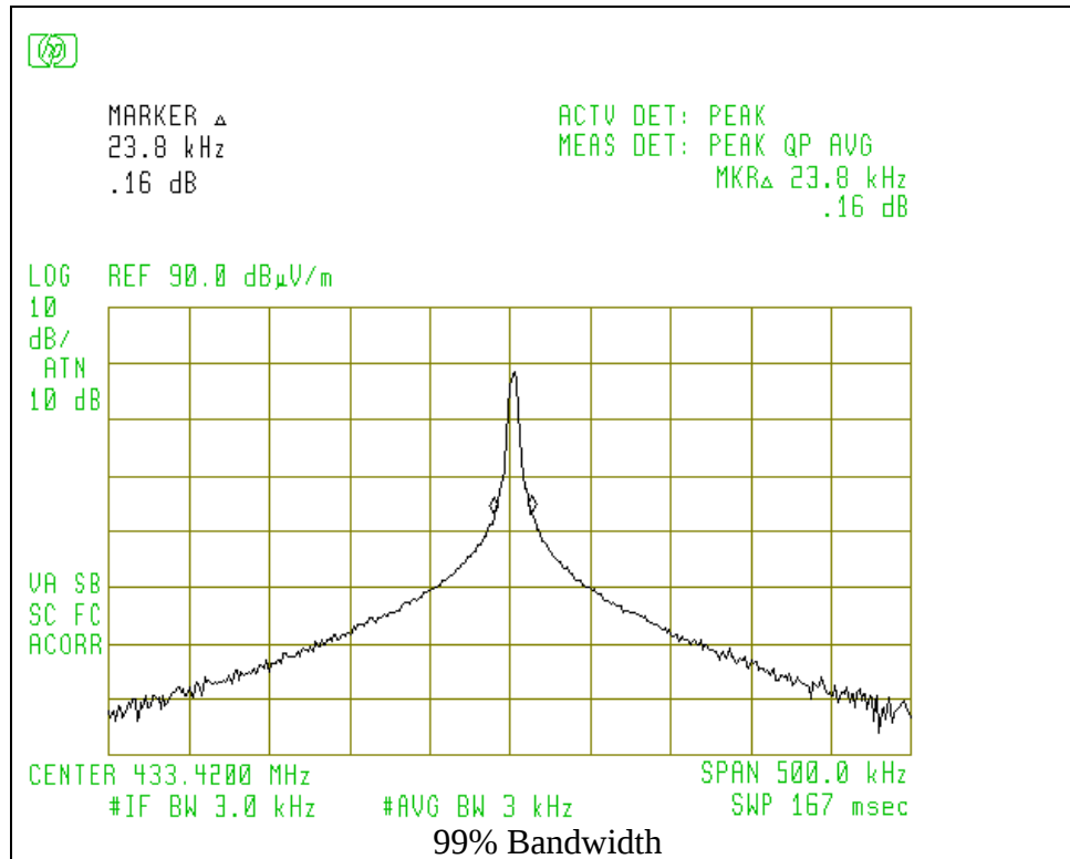
Figure 6.1 Occupied Bandwidth
