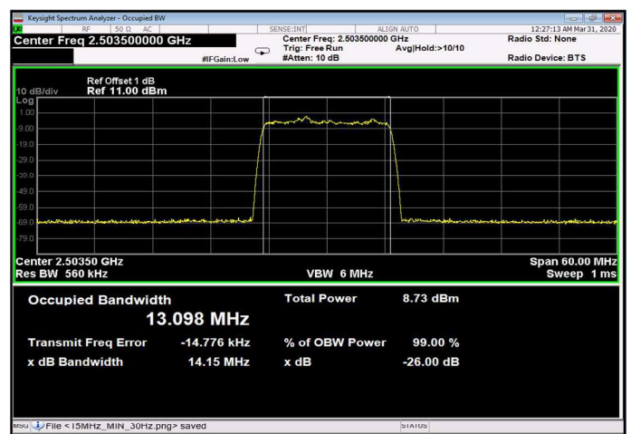
Figure 218: 64QAM 15MHz B.W.; 2503.5 MHz, 60kHz Input
