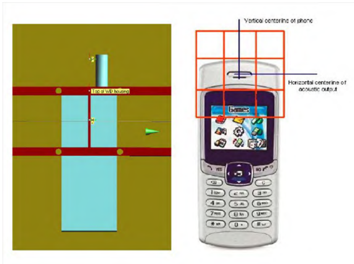
Fig. 3 WD reference and plane for RF emission measurements
