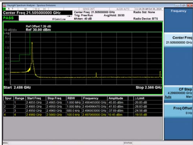
NTNV-n41-PC2-30-70-L-DFT-BPSK-Edge_1RB_Left-PASS
