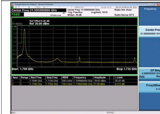
NTNV-n66-PC3-15-25-L-DFT-BPSK-Edge_1RB_Left-PASS
