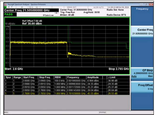
NTVN-n41-PC2-30-90-H-DFT-BPSK-Outer_Full-PASS
