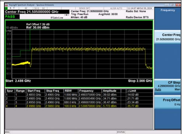
NTNV-n41-PC2-30-70-L-DFT-BPSK-Outer_Full-PASS
