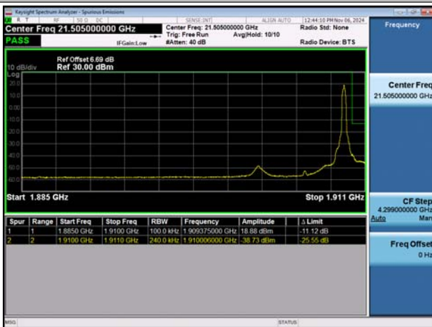
NTNV-n2-PC3-15-25-H-DFT-BPSK-Edge_1RB_Right-PASS
