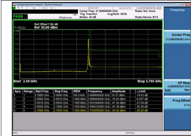
NTVN-n41-PC2-30-100-H-DFT-BPSK-Edge_1RB_Right-PASS
