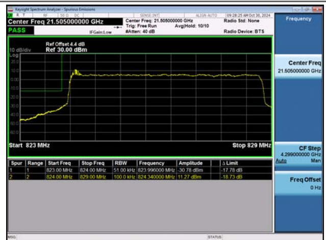
NTVN-n5-PC3-15-5-L-DFT-BPSK-Outer_Full-PASS
