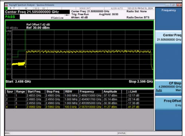
NTVN-n41-PC2-30-100-L-DFT-BPSK-Outer_Full-PASS
