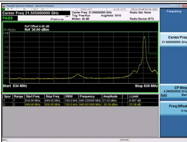
NTNV-n5-PC3-15-15-H-DFT-BPSK-Edge_1RB_Right-PASS
