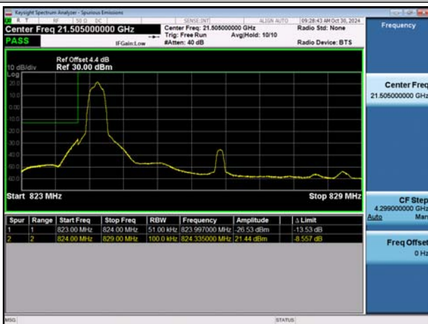
NTVN-n5-PC3-15-5-L-DFT-BPSK-Edge_1RB_Left-PASS
