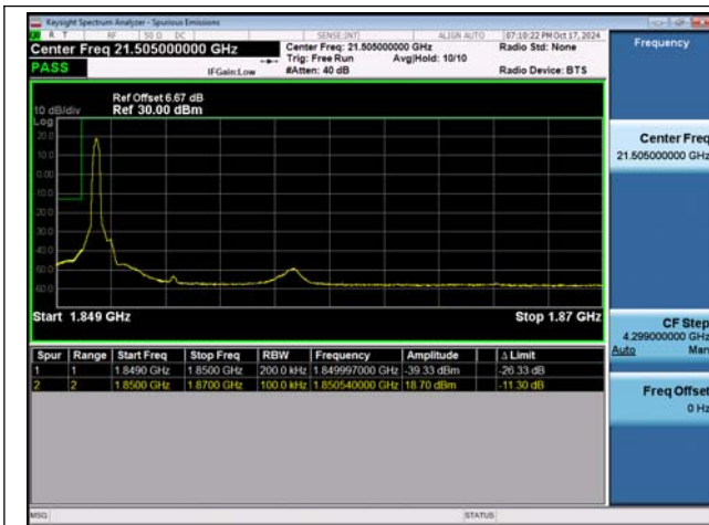
NTVN-n2-PC3-15-20-L-DFT-BPSK-Edge_1RB_Left-PASS
