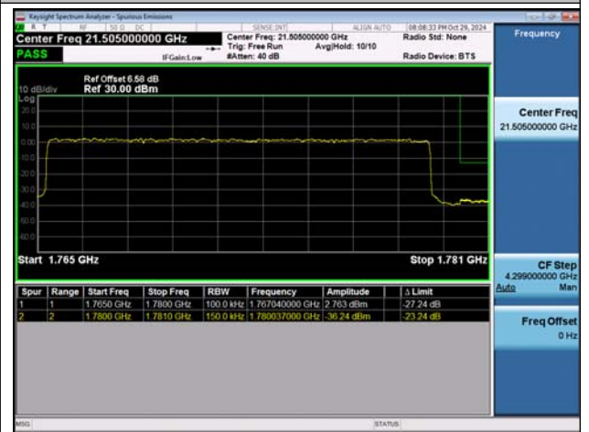
NTNV-n66-PC3-15-15-H-DFT-BPSK-Outer_Full-PASS
