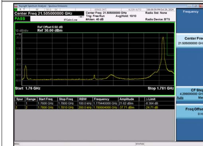
NTNV-n66-PC3-15-20-H-DFT-BPSK-Edge_1RB_Right-PASS
