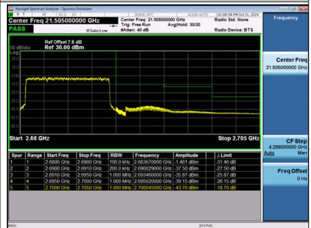
NTNV-n41-PC2-30-10-H-DFT-BPSK-Outer_Full-PASS
