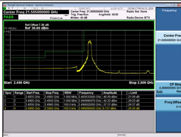
NTNV-n41-PC2-30-10-L-DFT-BPSK-Edge_1RB_Left-PASS
