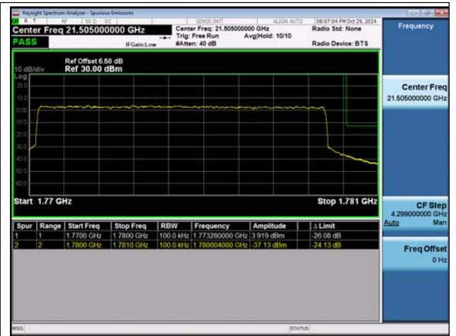
NTNV-n66-PC3-15-10-H-DFT-BPSK-Outer_Full-PASS
