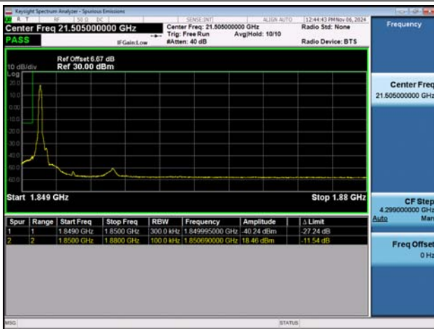
NTNV-n2-PC3-15-30-L-DFT-BPSK-Edge_1RB_Left-PASS
