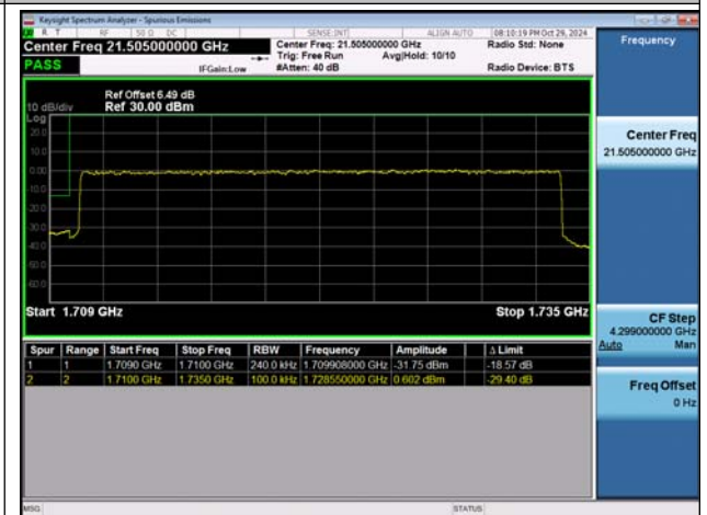
NTNV-n66-PC3-15-25-L-DFT-BPSK-Outer_Full-PASS
