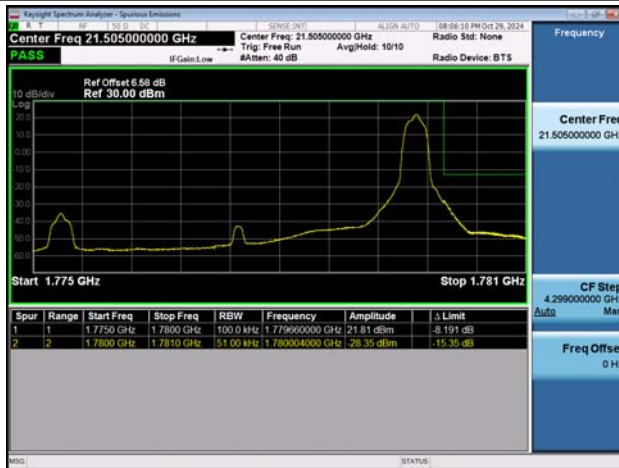
NTNV-n66-PC3-15-5-H-DFT-BPSK-Edge_1RB_Right-PASS
