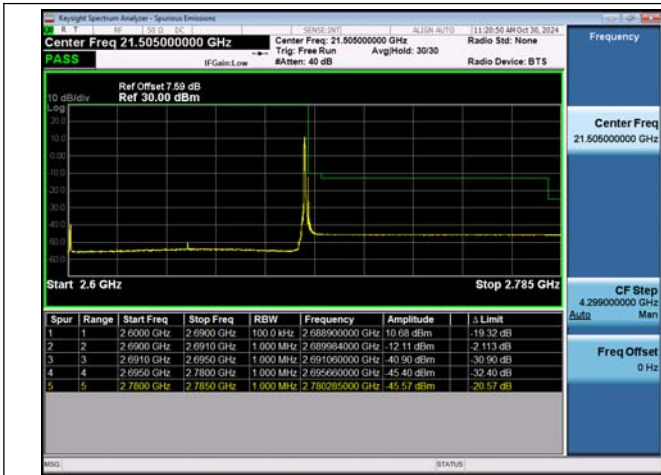
NTVN-n41-PC2-30-90-H-DFT-BPSK-Edge_1RB_Right-PASS
