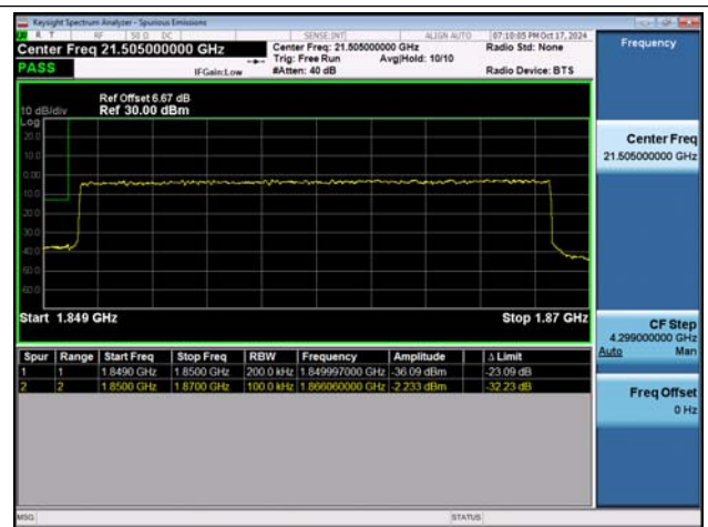
NTVN-n2-PC3-15-20-L-DFT-BPSK-Outer_Full-PASS
