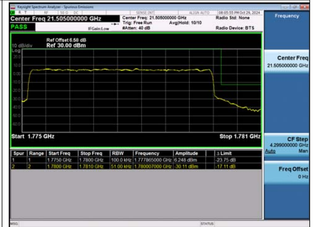
NTNV-n66-PC3-15-5-H-DFT-BPSK-Outer_Full-PASS
