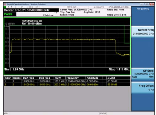
NTVN-n2-PC3-15-20-H-DFT-BPSK-Outer_Full-PASS
