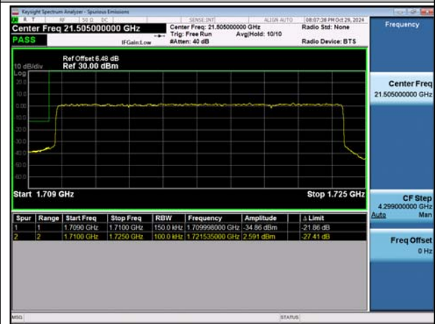
NTNV-n66-PC3-15-15-L-DFT-BPSK-Outer_Full-PASS
