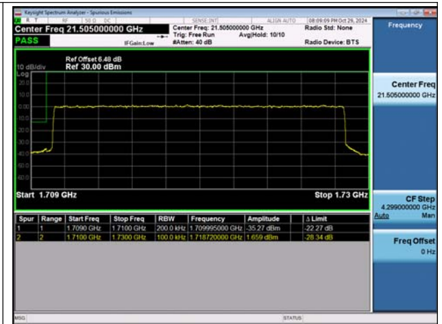
NTNV-n66-PC3-15-20-L-DFT-BPSK-Outer_Full-PASS
