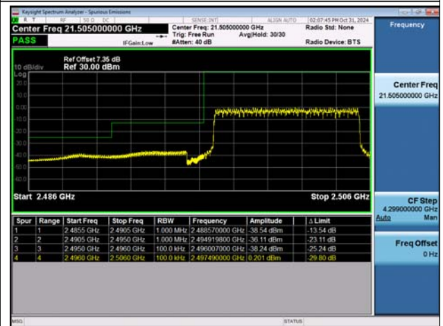
NTNV-n41-PC2-30-10-L-DFT-BPSK-Outer_Full-PASS
