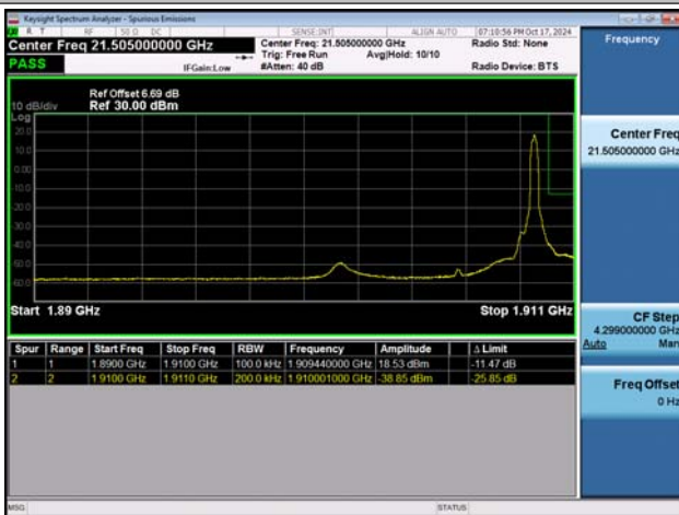
NTVN-n2-PC3-15-20-H-DFT-BPSK-Edge_1RB_Right-PASS
