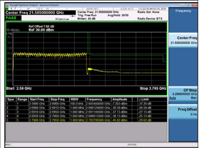
NTVN-n41-PC2-30-100-H-DFT-BPSK-Outer_Full-PASS
