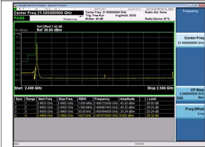
NTVN-n41-PC2-30-100-L-DFT-BPSK-Edge_1RB_Left-PASS
