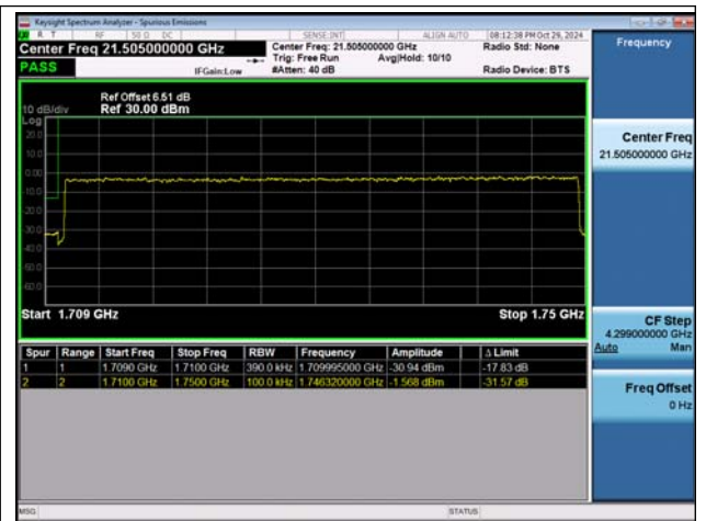
NTNV-n66-PC3-15-40-L-DFT-BPSK-Outer_Full-PASS
