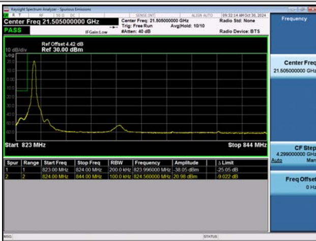
NTNV-n5-PC3-15-20-L-DFT-BPSK-Edge_1RB_Left-PASS
