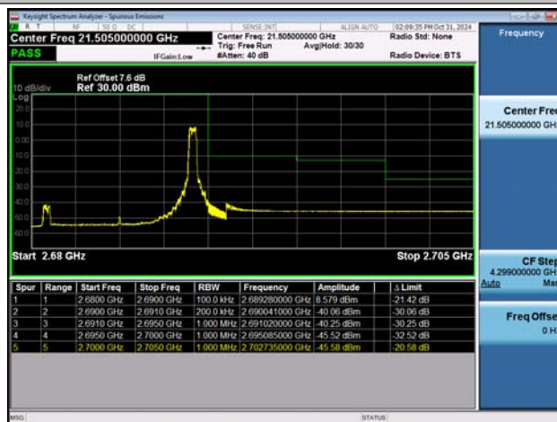
NTNV-n41-PC2-30-10-H-DFT-BPSK-Edge_1RB_Right-PASS
