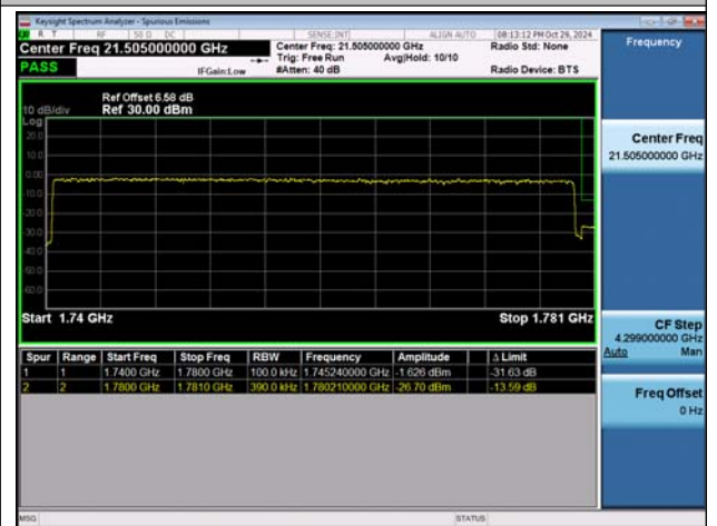
NTNV-n66-PC3-15-40-H-DFT-BPSK-Outer_Full-PASS
