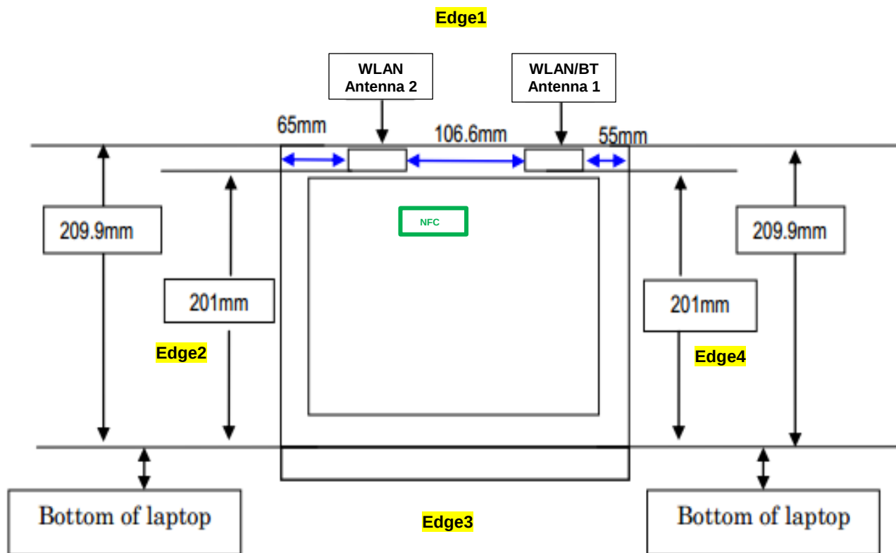
Front View
