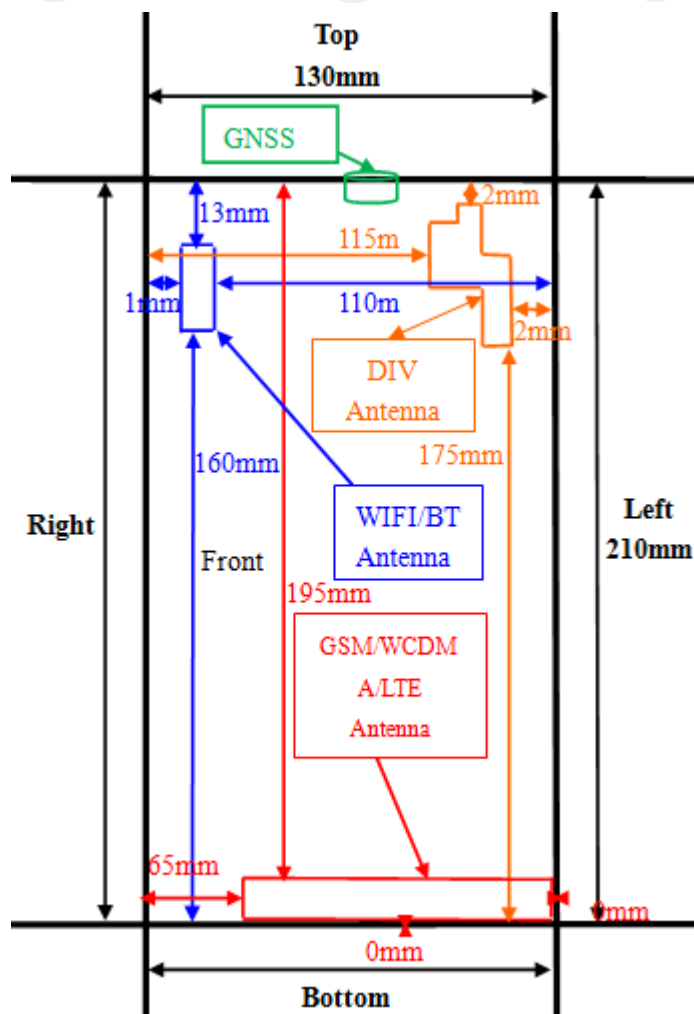
Antenna Configuration 1- LT800H
