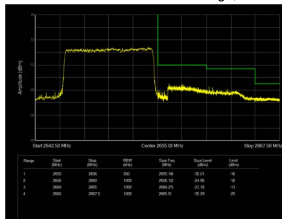
LTE Band 41 QPSK 15MHz CH-High, 1 RB
