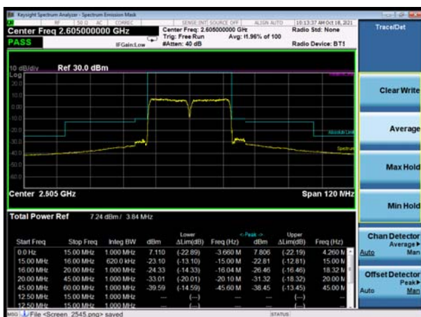
CA_38C 64QAM 15MHz+15MHz CH- High, RB 1
