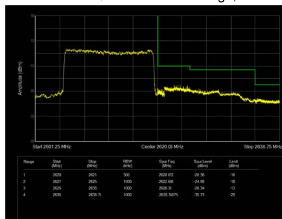
LTE Band 38 QPSK 15MHz CH-High, 100%RB
