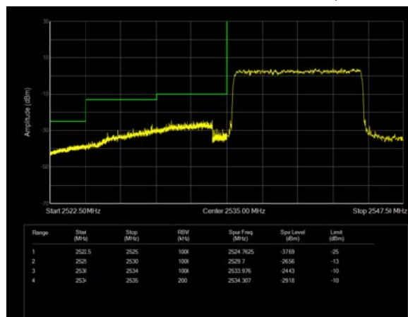
LTE Band 41 QPSK 15MHz CH-Low, 1 RB
