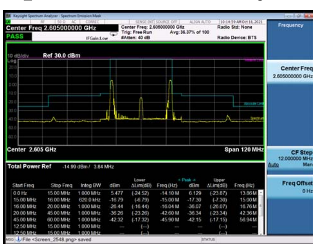
CA_38C 64QAM 15MHz+15MHz CH- High, 100%RB
