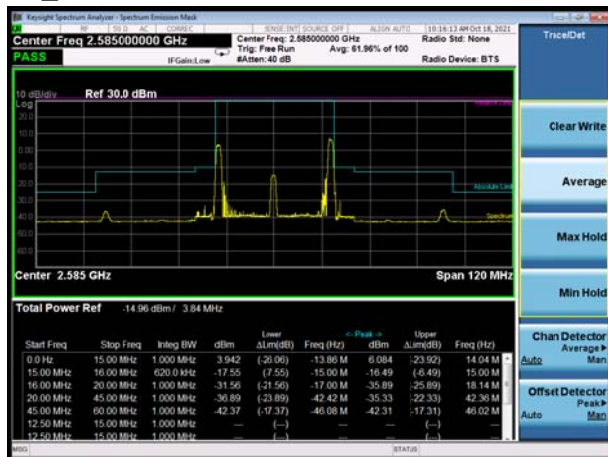
CA_38C 64QAM 15MHz+15MHz CH-Low, RB 1
