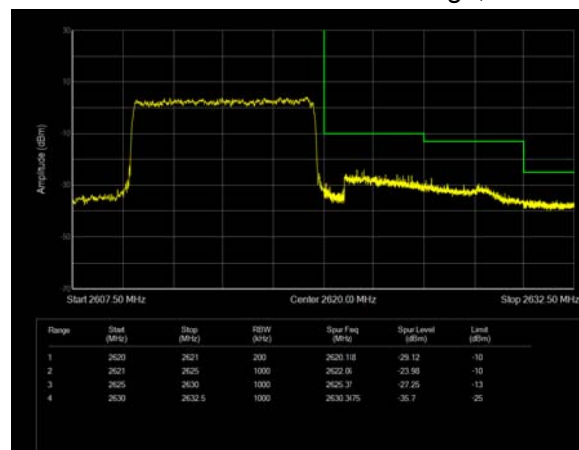
LTE Band 38 QPSK 15MHz CH-High, 1 RB
