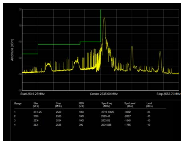
LTE Band 41 QPSK 15MHz CH-Low, 100%RB
