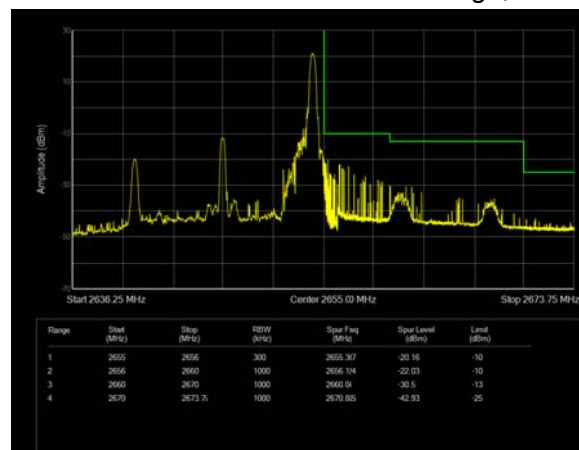
LTE Band 41 QPSK 15MHz CH-High, 100%RB
