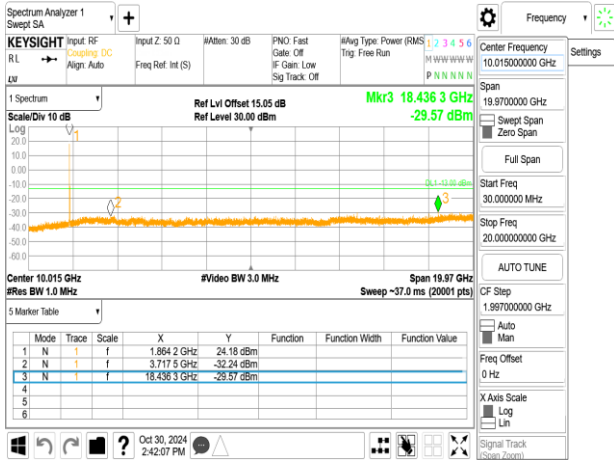
Band2_15MHz+15MHz_QPSK_RB1-74_1-0_CH18825-18975
