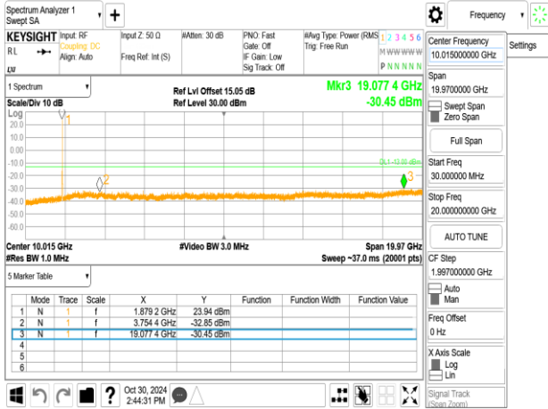
Band2_15MHz+15MHz_QPSK_RB1-74_1-0_CH18975-19125
