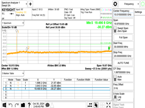
Band2_15MHz+15MHz_QPSK_RB1-74_1-0_CH18975-19125
