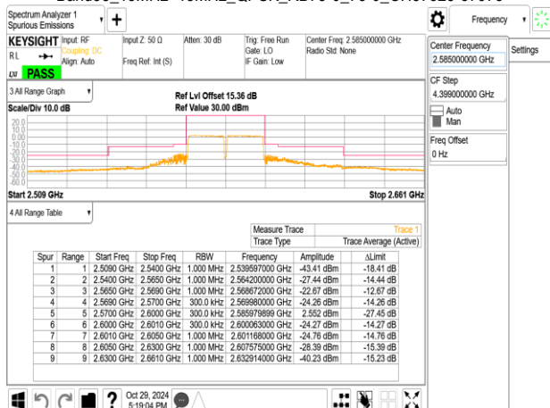
Band38_15MHz+15MHz_QPSK_RB75-0_75-0_CH37925-38075
