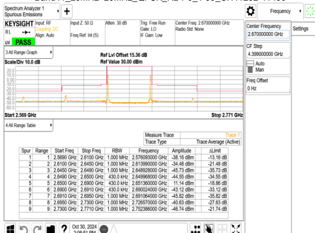
Band41_20MHz+20MHz_QPSK_RB100-0_100-0_CH39750-39948
