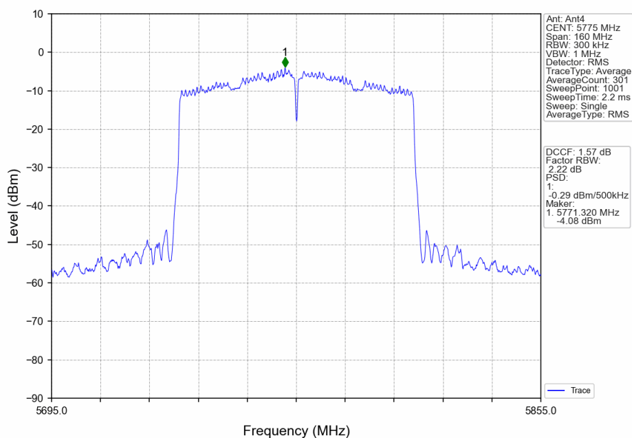
802.11ac(VHT80)_MCH_5775MHz_Ant4_NTNV
