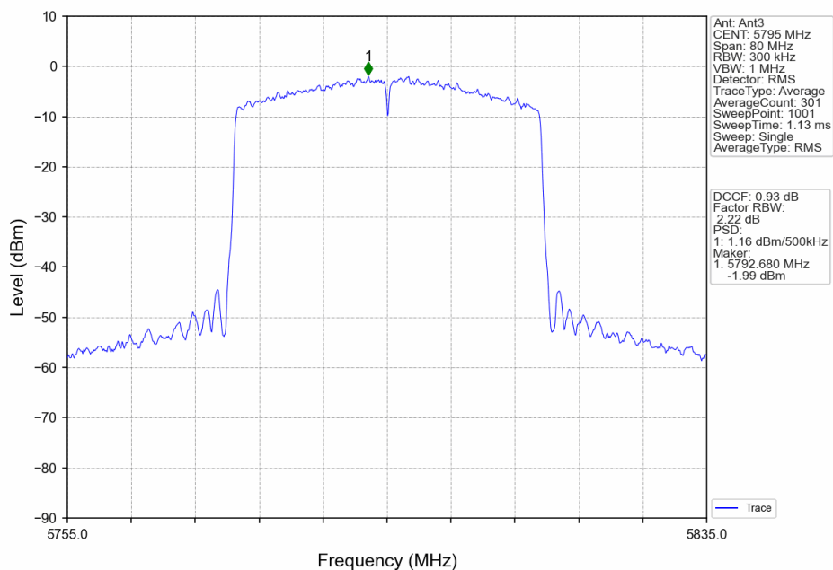
802.11ax(HEW40)_HCH_5795MHz_RU484_Left_Ant3_NTNV
