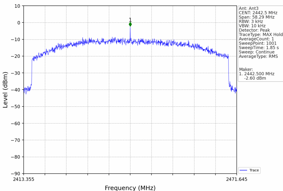
60M_HCH_2442.5MHz_Ant3_NTNV
