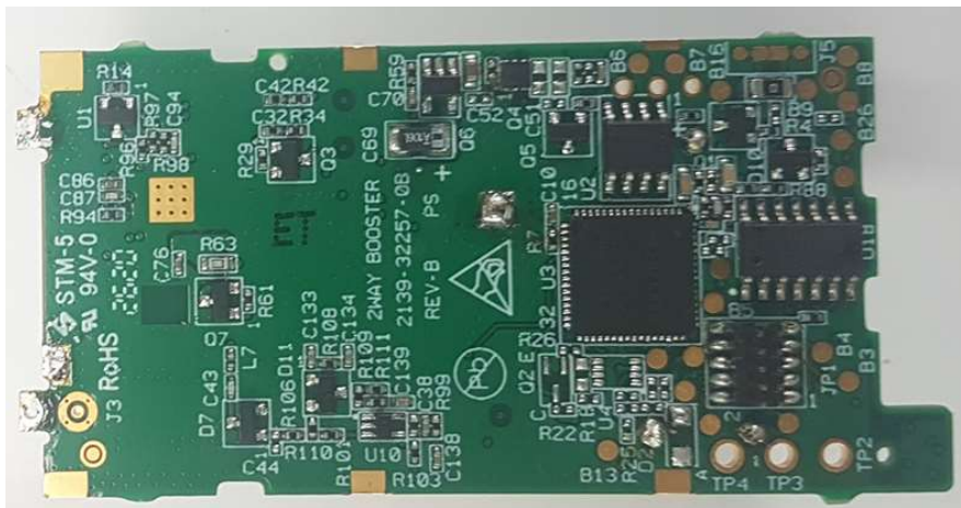
RF card - bottom view
