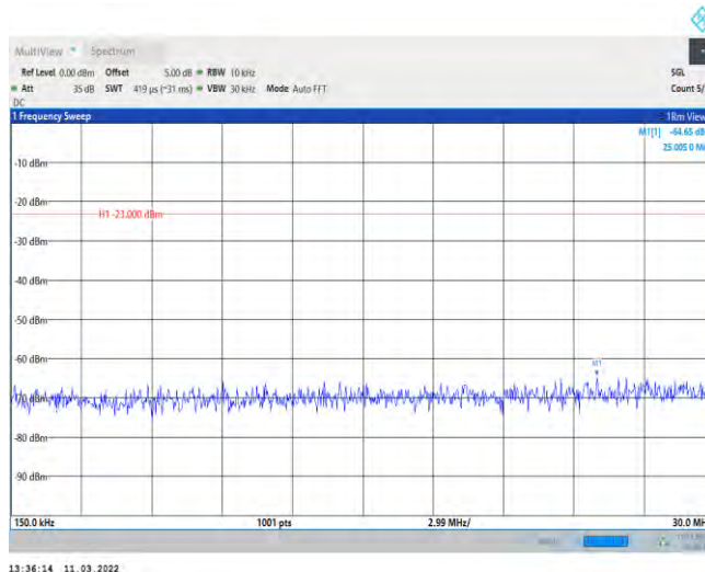
Band5-10MHz-QPSK-20450-1RB#0-Range2:0.15~30MHz
