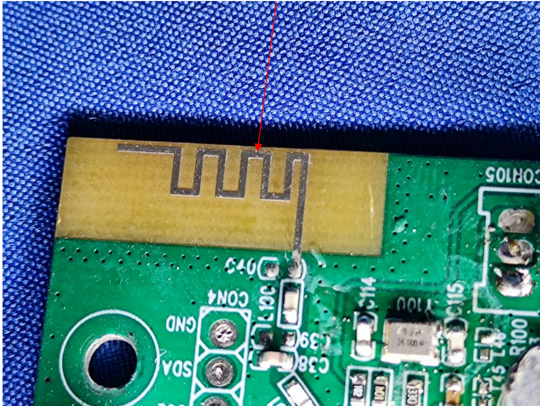
Bluetooth Antenna
