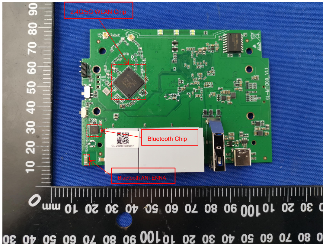
MAIN BOARD TOP VIEW(WITHOUT SHIELDING)
