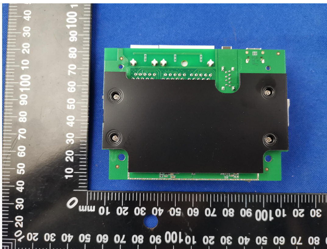
MAIN BOARD BACK VIEW(WITH SHIELDING)
