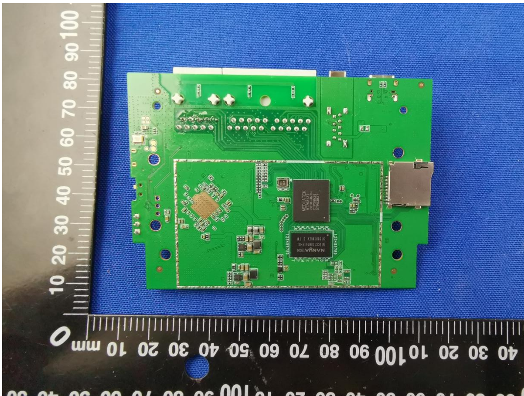
MAIN BOARD BACK VIEW(WITHOUT SHIELDING)
