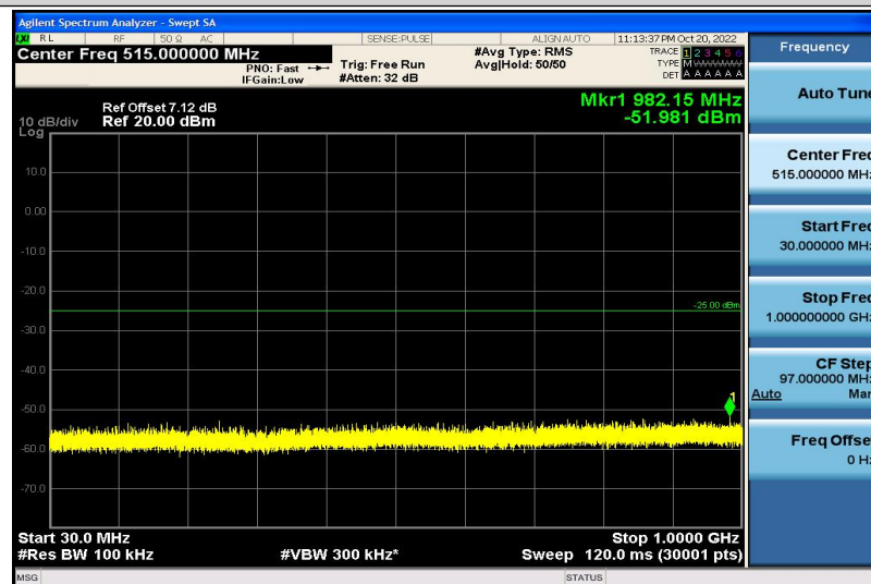
Band7-20MHz-16QAM-21100-1RB#0-30~1000MHz
