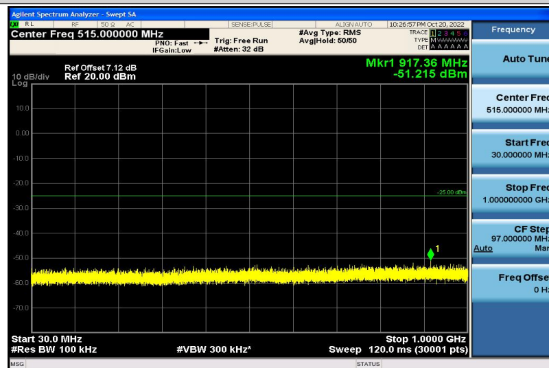
Band7-10MHz-16QAM-21100-1RB#0-30~1000MHz
