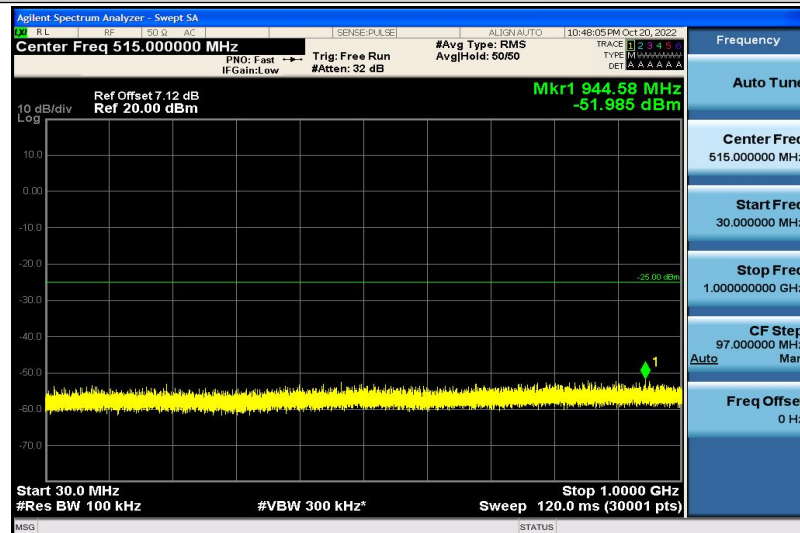
Band7-15MHz-QPSK-21100-1RB#0-30~1000MHz
