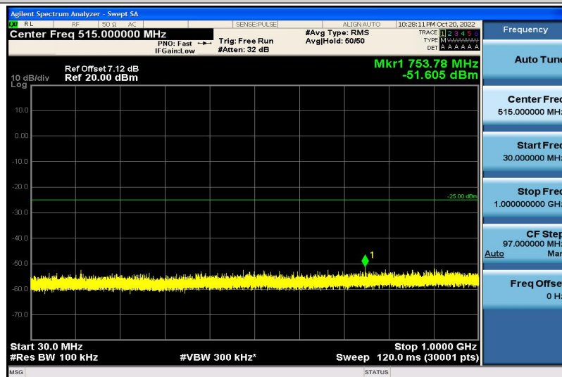
Band7-10MHz-16QAM-21400-1RB#0-30~1000MHz
