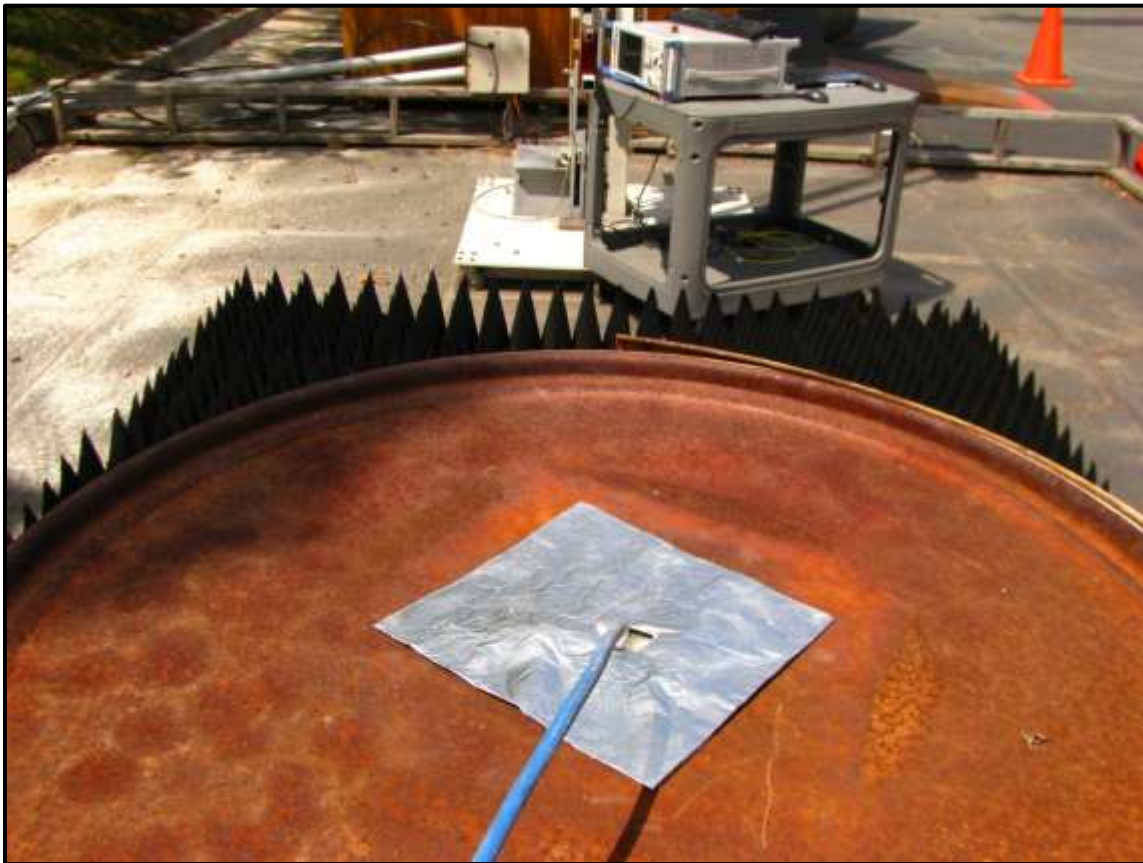
Photograph 22: Radiated Emissions – TC #2 Swivel; Steel Container, Rear View
