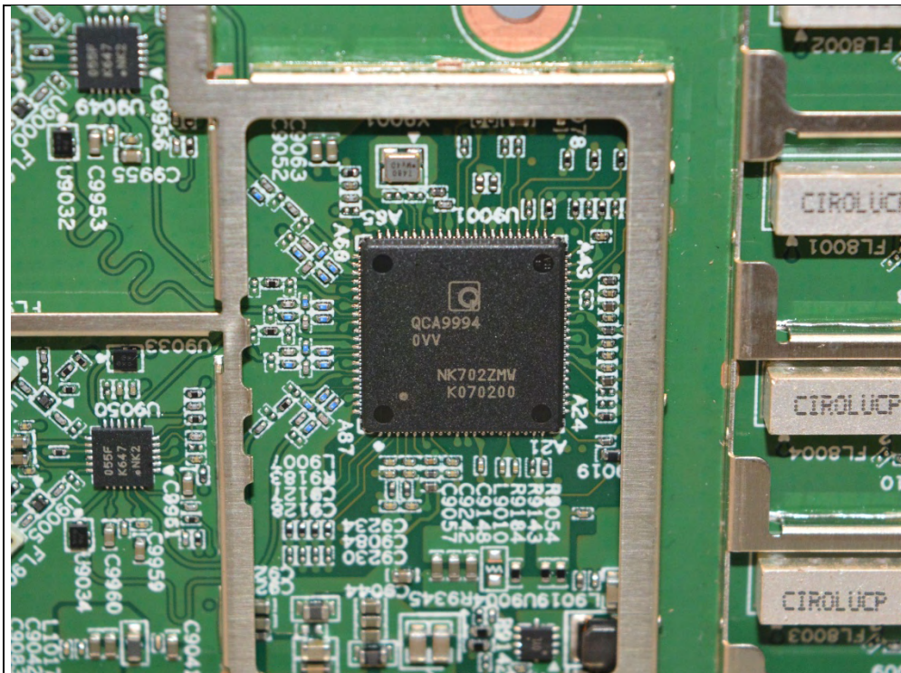
RF chipset for WLAN 2.4G
