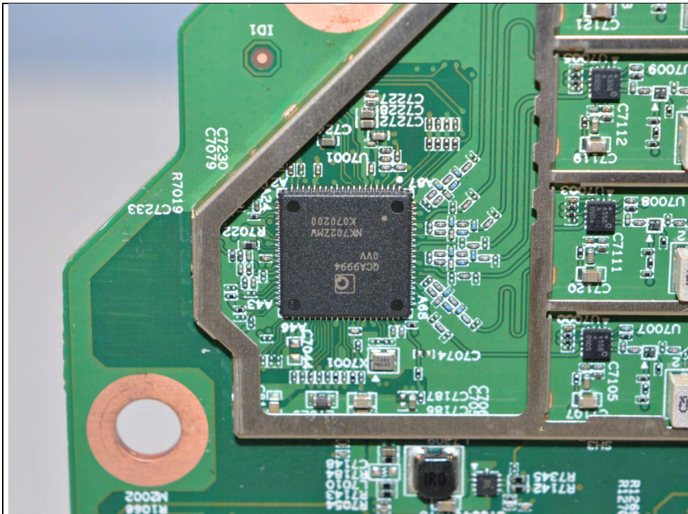
RF chipset for WLAN 5G (5.18-5.24GHz)
