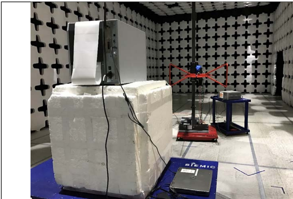
Radiated Emissions (<1GHz) – Front View
