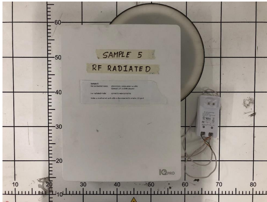
1. Front view of the DUT
