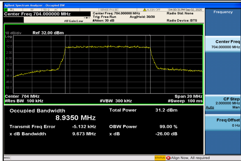
Band12-10MHz-QPSK-23060-50RB#0-8.9350
