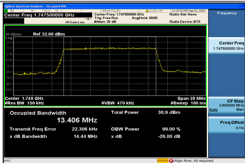
Band4-15MHz-QPSK-20325-75RB#0-13.406
