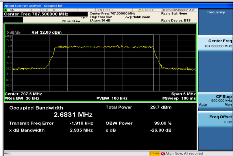
Band12-3MHz-16QAM-23095-15RB#0-2.6831
