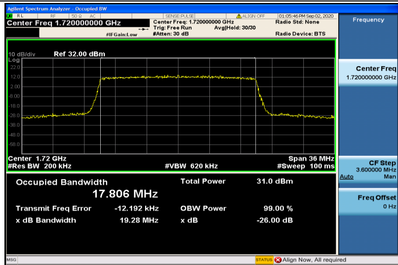
Band4-20MHz-QPSK-20050-100RB#0-17.806
