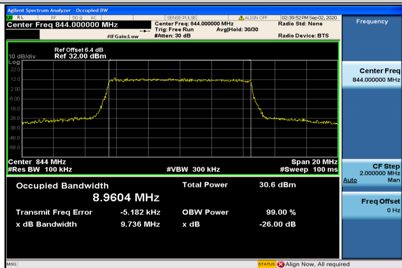
Band5-10MHz-QPSK-20600-50RB#0-8.9604
