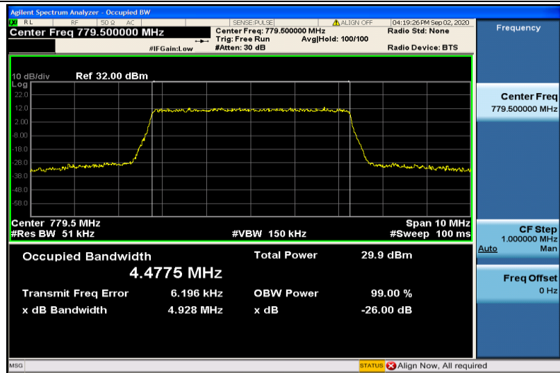
Band13-5MHz-16QAM-23205-25RB#0-4.4775
