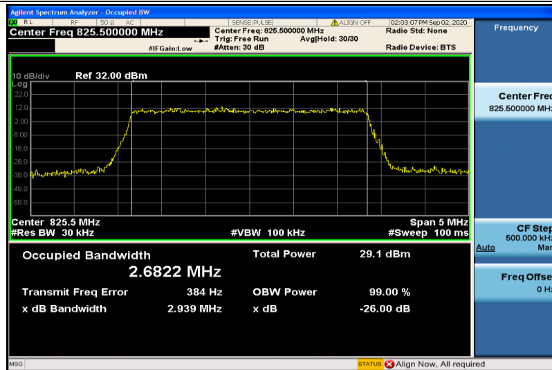
Band5-3MHz-16QAM-20415-15RB#0-2.6822
