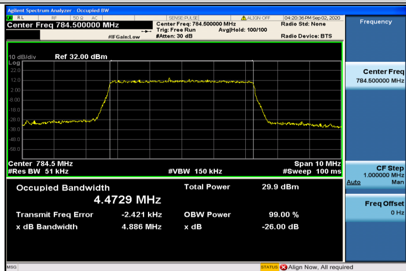
Band13-5MHz-16QAM-23255-25RB#0-4.4729
