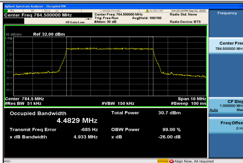
Band13-5MHz-QPSK-23255-25RB#0-4.4829
