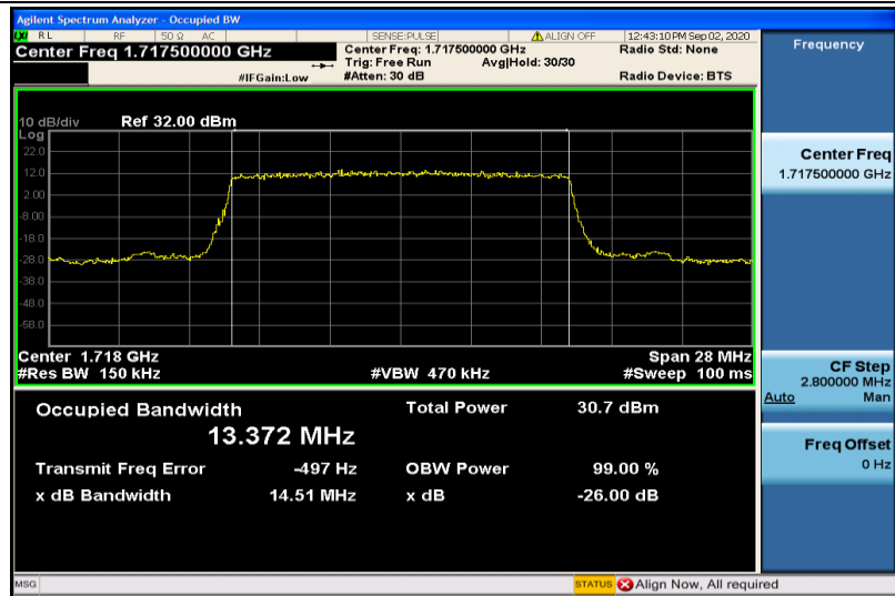
Band4-15MHz-QPSK-20025-75RB#0-13.372
