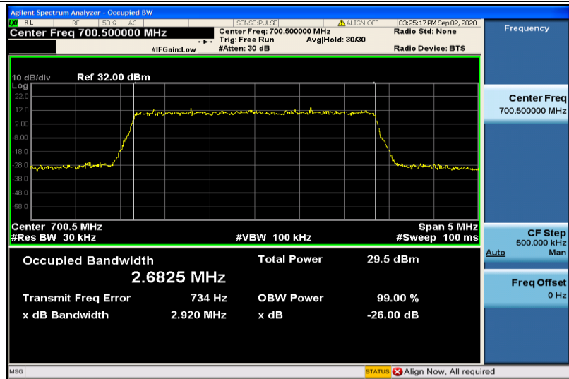
Band12-3MHz-16QAM-23025-15RB#0-2.6825
