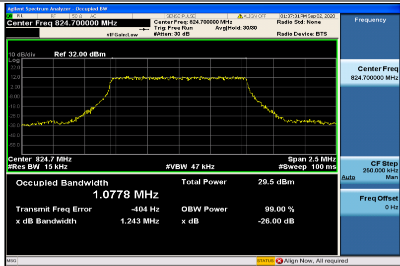
Band5-1.4MHz-QPSK-20407-6RB#0-1.0778
