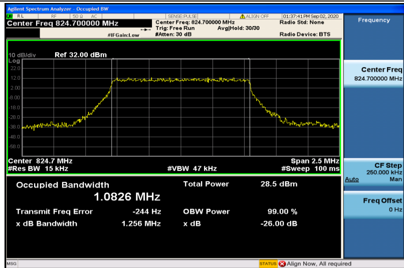
Band5-1.4MHz-16QAM-20407-6RB#0-1.0826
