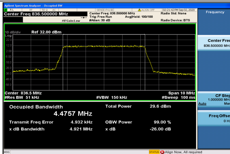
Band5-5MHz-16QAM-20525-25RB#0-4.4757
