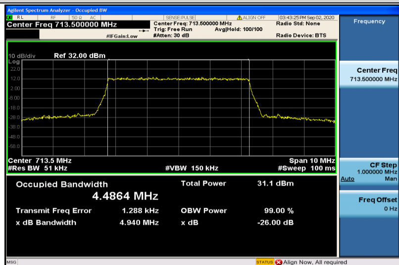
Band12-5MHz-QPSK-23155-25RB#0-4.4864
