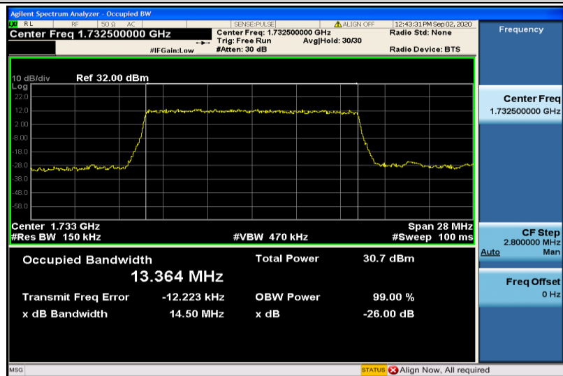
Band4-15MHz-QPSK-20175-75RB#0-13.364
