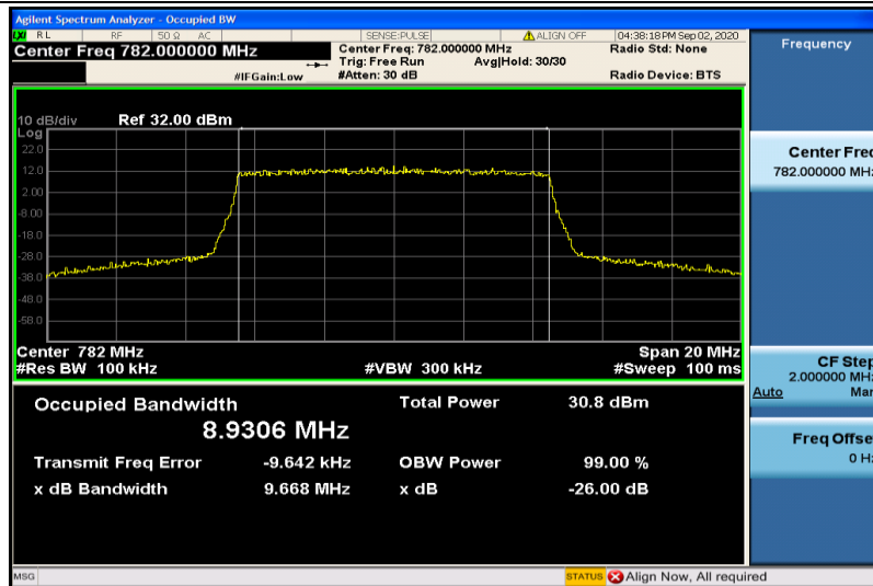
Band13-10MHz-QPSK-23230-50RB#0-8.9306
