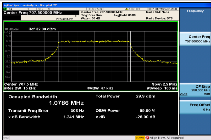
Band12-1.4MHz-QPSK-23095-6RB#0-1.0786
