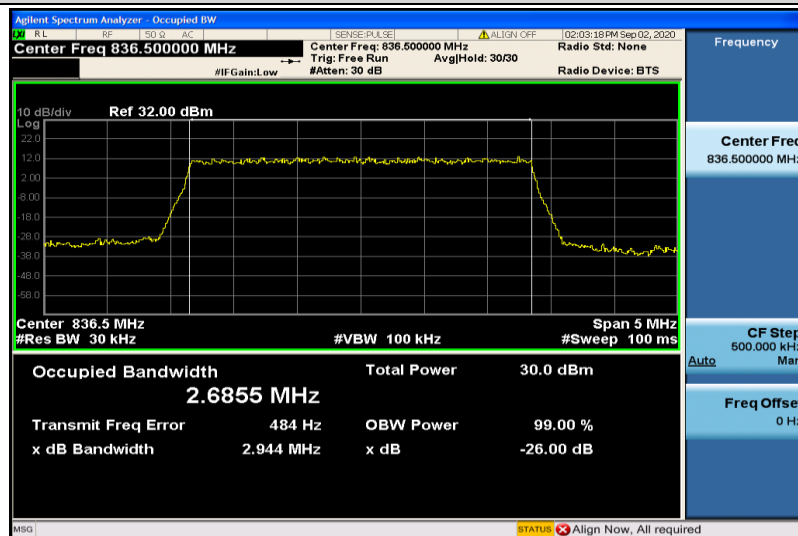
Band5-3MHz-QPSK-20525-15RB#0-2.6855
