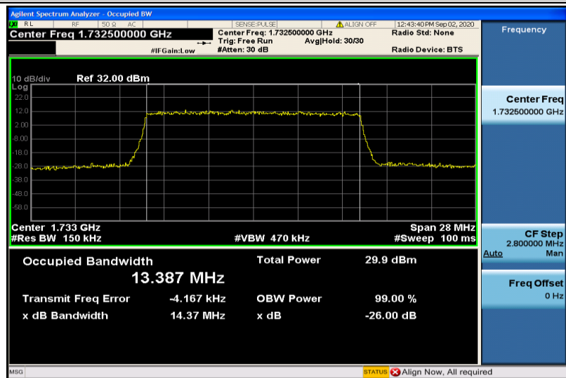
Band4-15MHz-16QAM-20175-75RB#0-13.387
