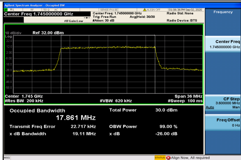
Band4-20MHz-16QAM-20300-100RB#0-17.861
