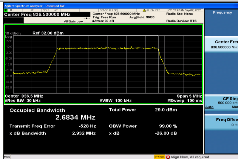
Band5-3MHz-16QAM-20525-15RB#0-2.6834
