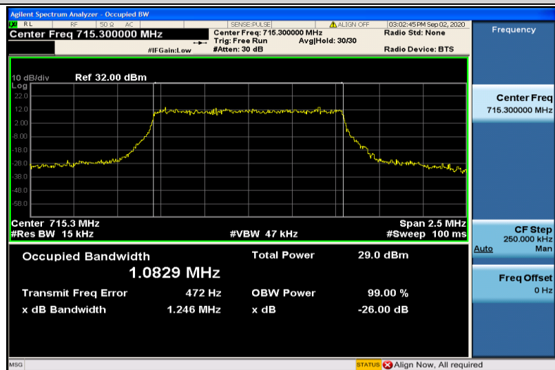
Band12-1.4MHz-16QAM-23173-6RB#0-1.0829
