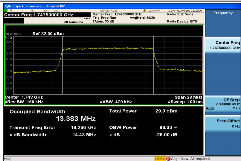
Band4-15MHz-16QAM-20325-75RB#0-13.383
