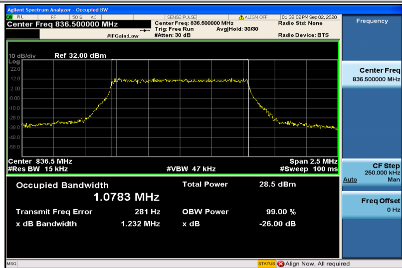
Band5-1.4MHz-16QAM-20525-6RB#0-1.0783
