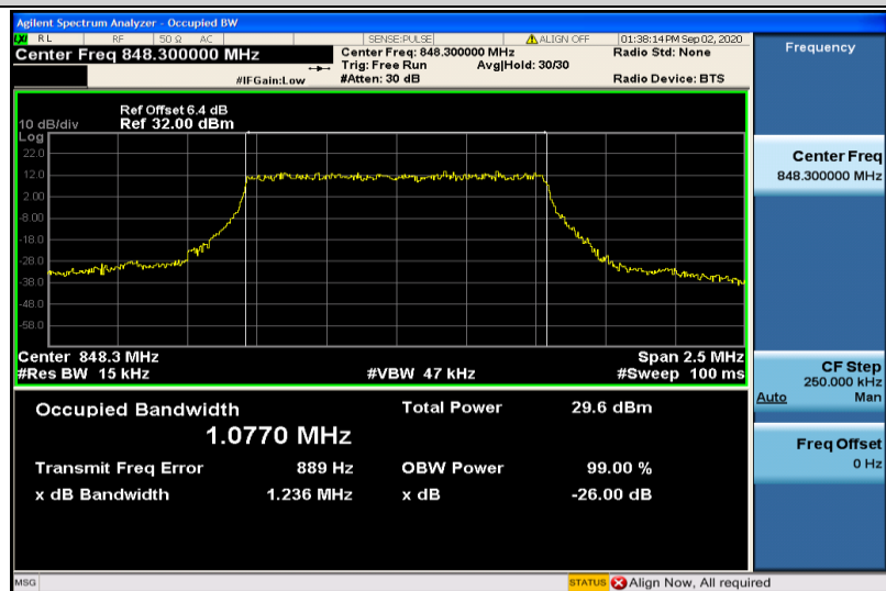
Band5-1.4MHz-QPSK-20643-6RB#0-1.0770
