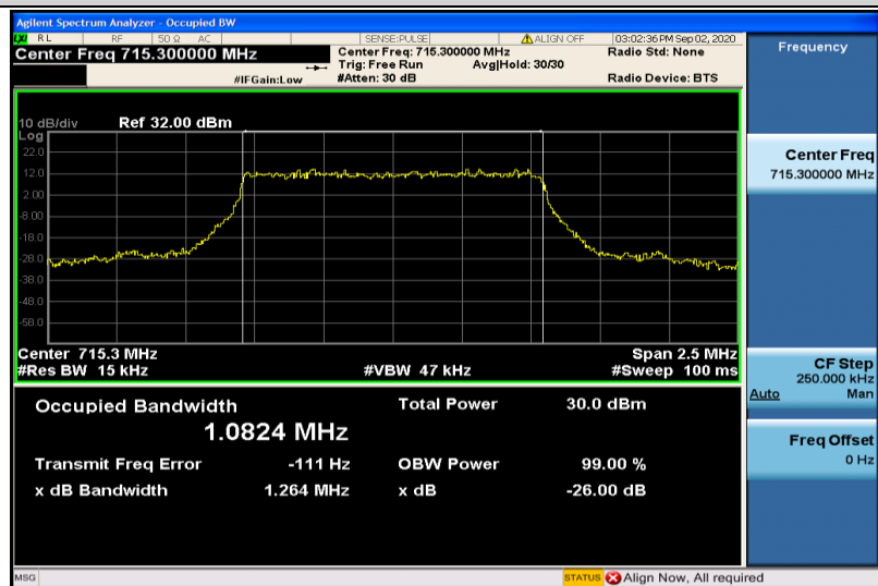
Band12-1.4MHz-QPSK-23173-6RB#0-1.0824
