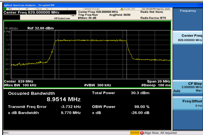
Band5-10MHz-QPSK-20450-50RB#0-8.9514
