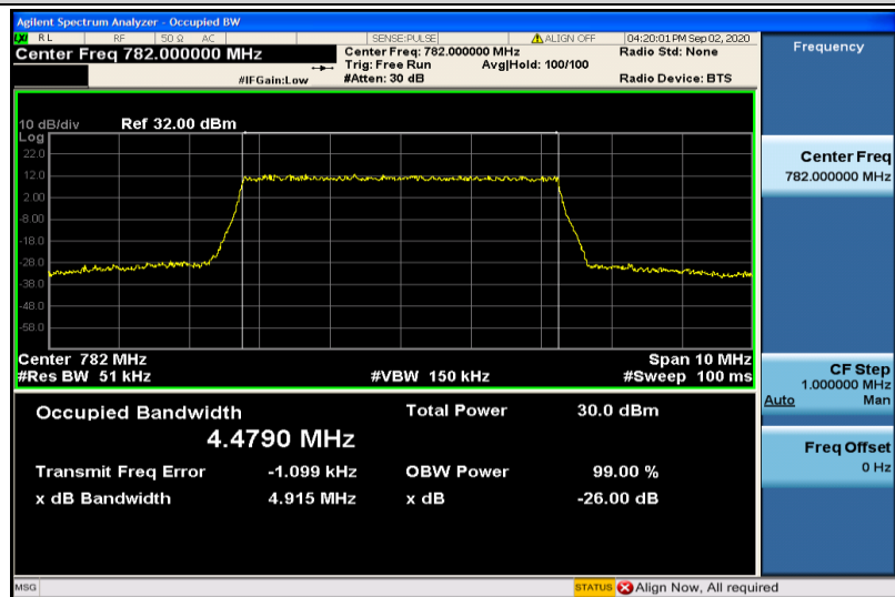
Band13-5MHz-16QAM-23230-25RB#0-4.4790
