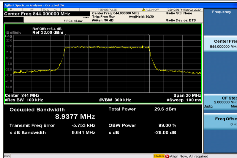
Band5-10MHz-16QAM-20600-50RB#0-8.9377
