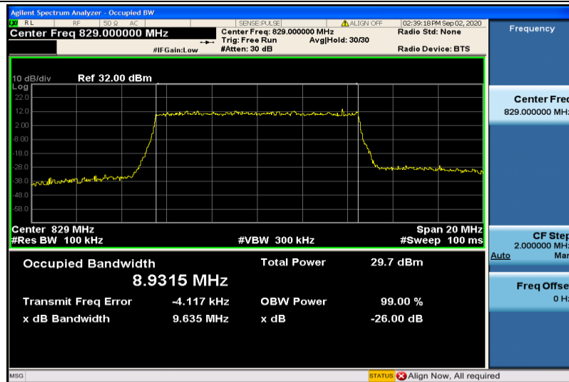
Band5-10MHz-16QAM-20450-50RB#0-8.9315
