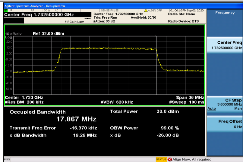
Band4-20MHz-16QAM-20175-100RB#0-17.867
