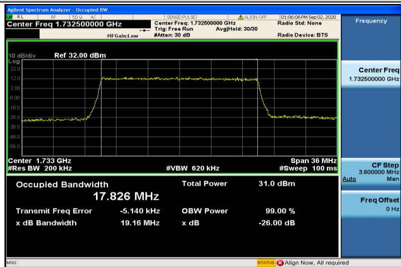
Band4-20MHz-QPSK-20175-100RB#0-17.826
