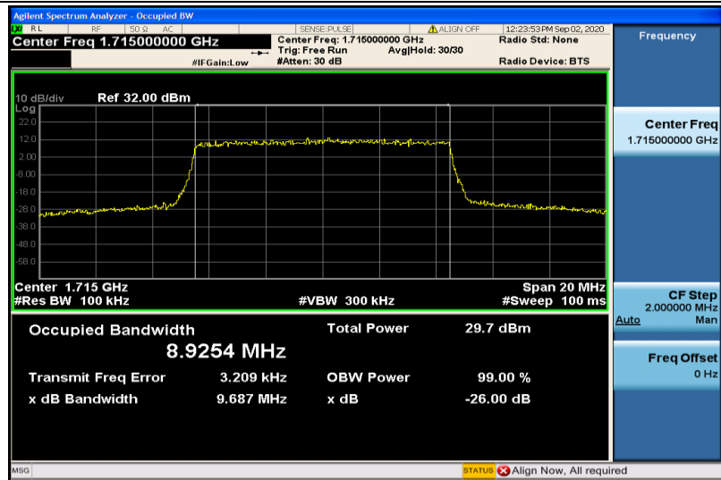
Band4-10MHz-16QAM-20000-50RB#0-8.9254
