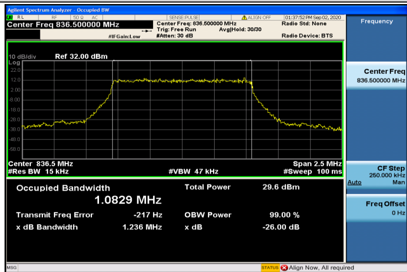
Band5-1.4MHz-QPSK-20525-6RB#0-1.0829
