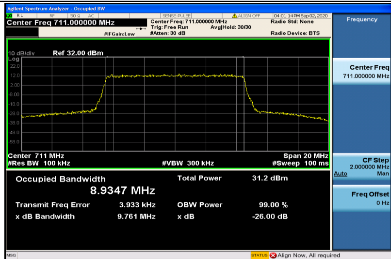
Band12-10MHz-QPSK-23130-50RB#0-8.9347
