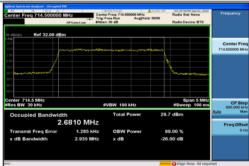
Band12-3MHz-16QAM-23165-15RB#0-2.6810
