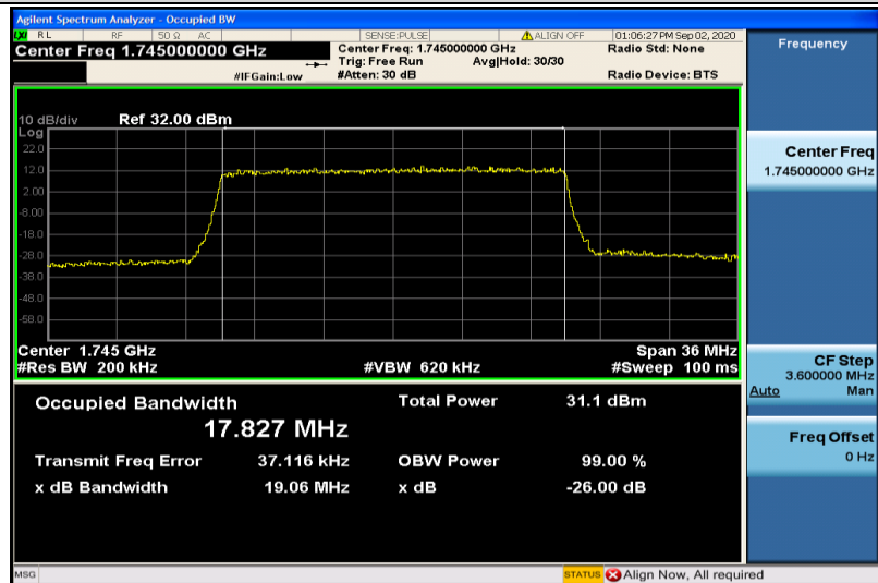
Band4-20MHz-QPSK-20300-100RB#0-17.827
