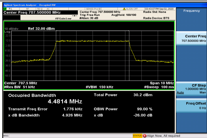
Band12-5MHz-16QAM-23095-25RB#0-4.4814
