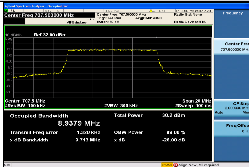
Band12-10MHz-16QAM-23095-50RB#0-8.9379
