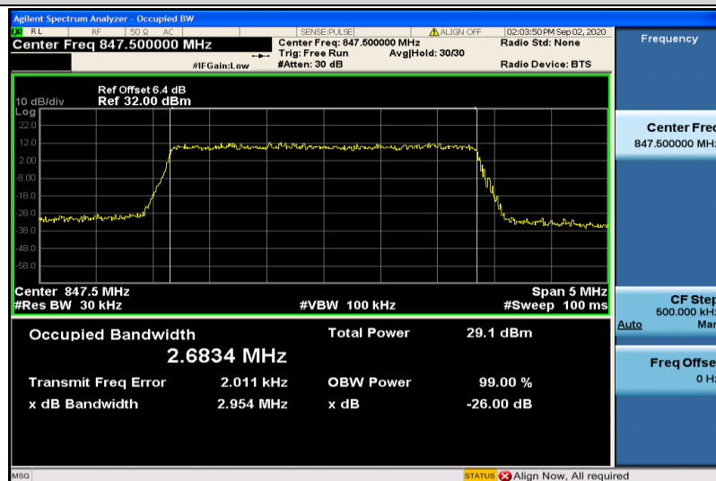
Band5-3MHz-16QAM-20635-15RB#0-2.6834
