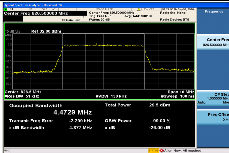
Band5-5MHz-16QAM-20425-25RB#0-4.4729
