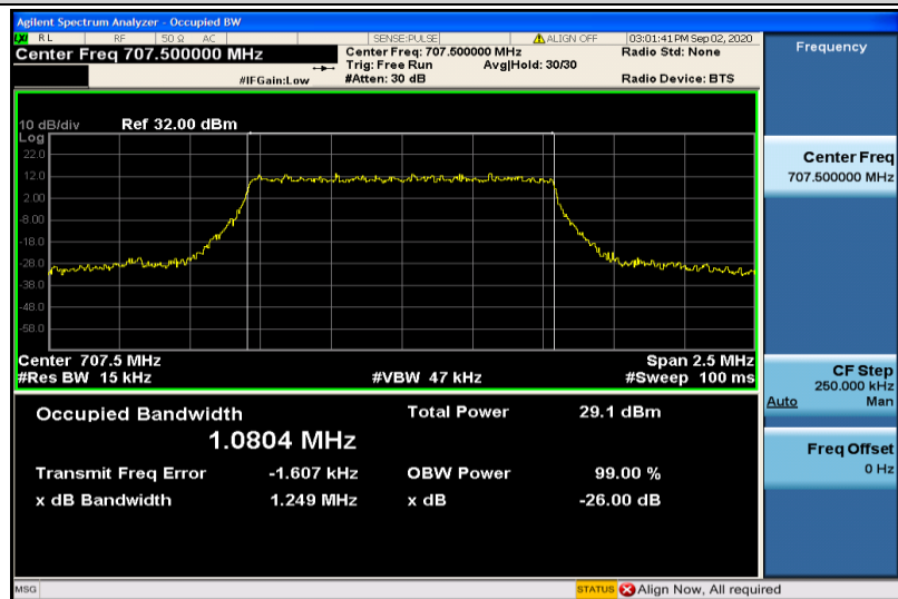
Band12-1.4MHz-16QAM-23095-6RB#0-1.0804
