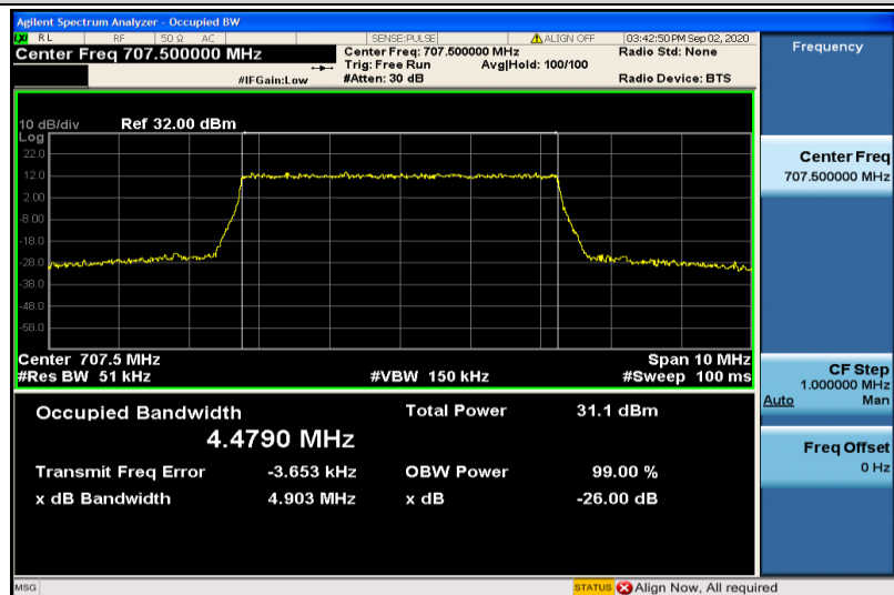
Band12-5MHz-QPSK-23095-25RB#0-4.4790
