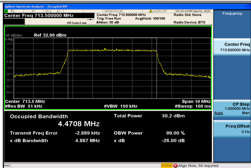
Band12-5MHz-16QAM-23155-25RB#0-4.4708
