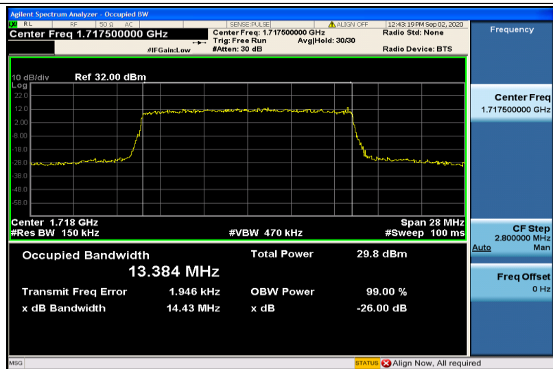
Band4-15MHz-16QAM-20025-75RB#0-13.384
