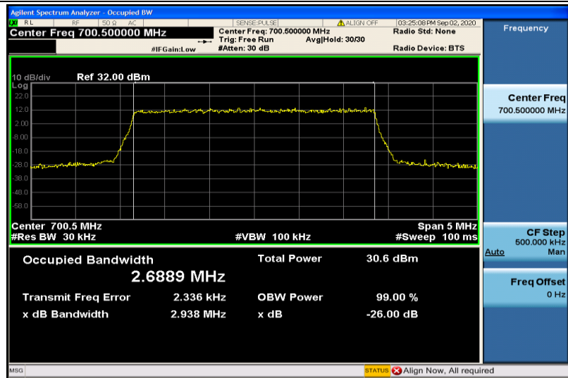
Band12-3MHz-QPSK-23025-15RB#0-2.6889
