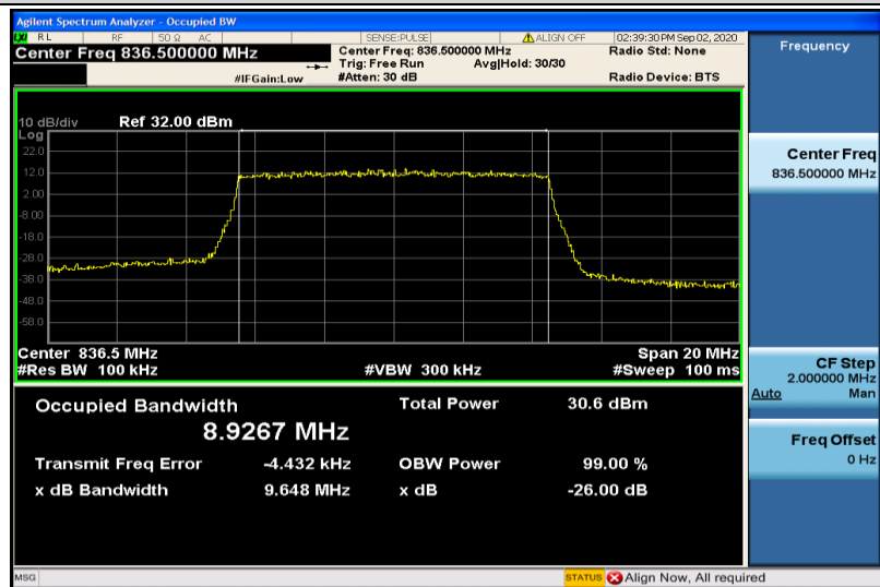
Band5-10MHz-QPSK-20525-50RB#0-8.9267
