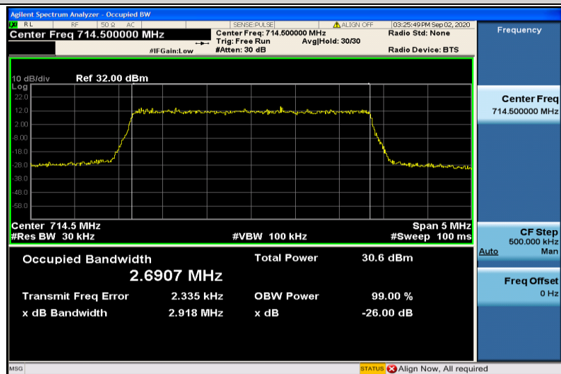
Band12-3MHz-QPSK-23165-15RB#0-2.6907
