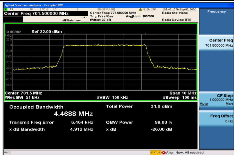
Band12-5MHz-QPSK-23035-25RB#0-4.4688
