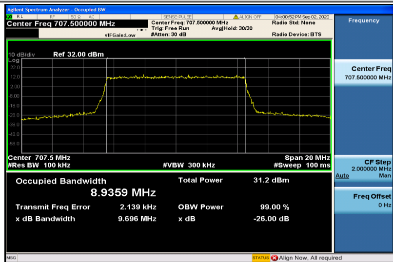
Band12-10MHz-QPSK-23095-50RB#0-8.9359
