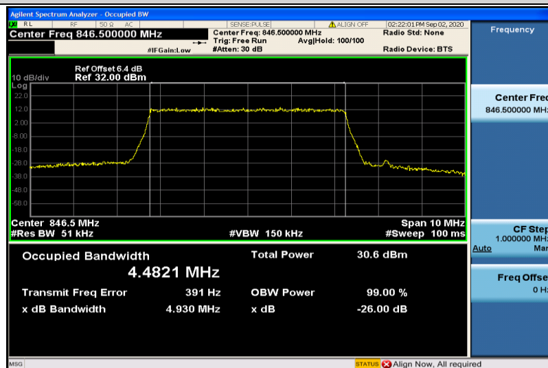
Band5-5MHz-QPSK-20625-25RB#0-4.4821
