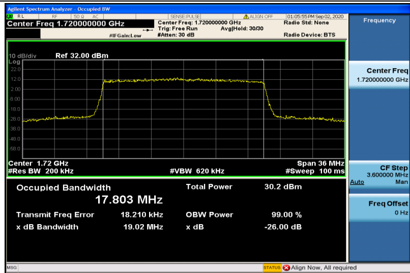
Band4-20MHz-16QAM-20050-100RB#0-17.803
