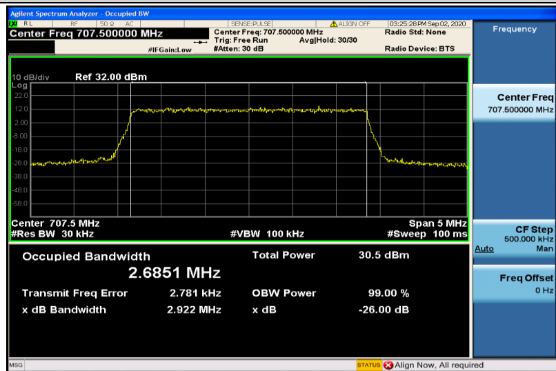
Band12-3MHz-QPSK-23095-15RB#0-2.6851
