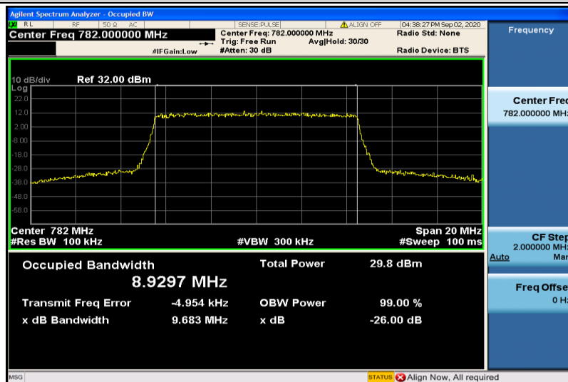
Band13-10MHz-16QAM-23230-50RB#0-8.9297
