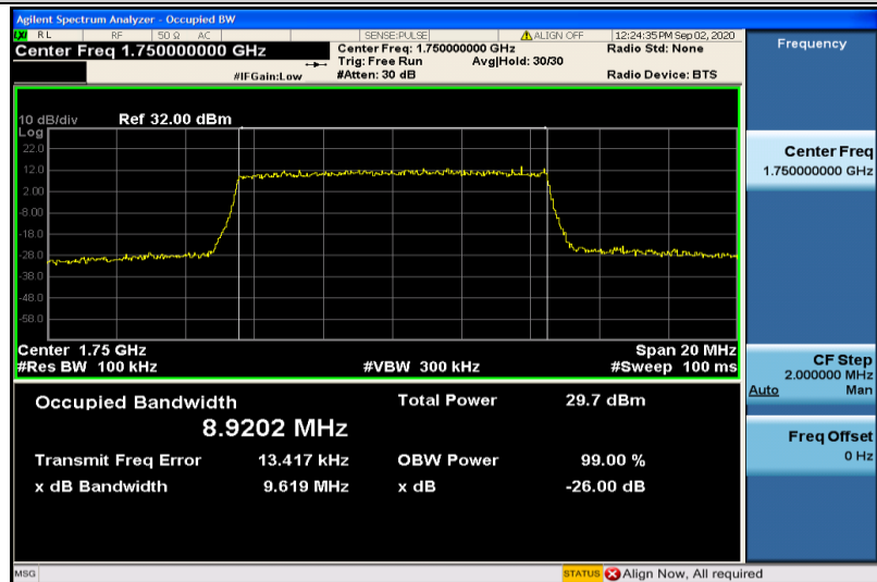
Band4-10MHz-16QAM-20350-50RB#0-8.9202
