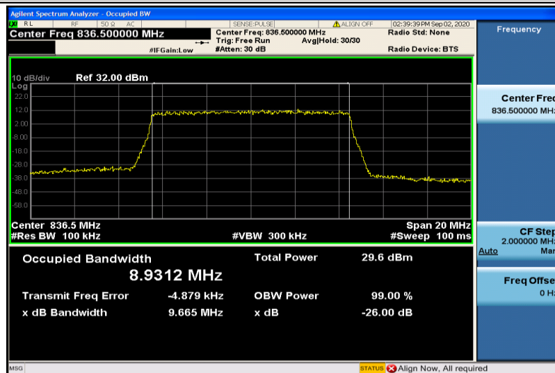
Band5-10MHz-16QAM-20525-50RB#0-8.9312
