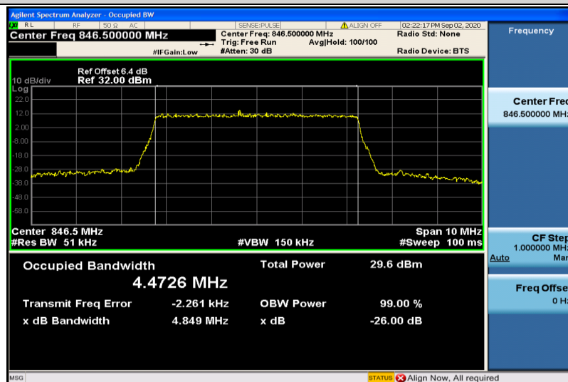
Band5-5MHz-16QAM-20625-25RB#0-4.4726
