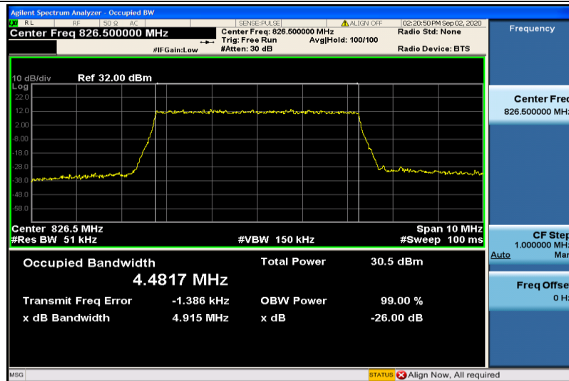
Band5-5MHz-QPSK-20425-25RB#0-4.4817
