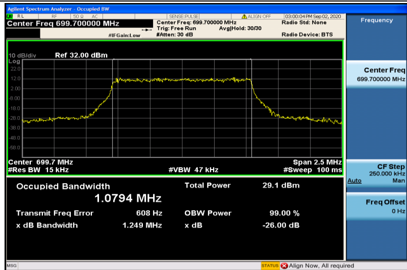
Band12-1.4MHz-16QAM-23017-6RB#0-1.0794
