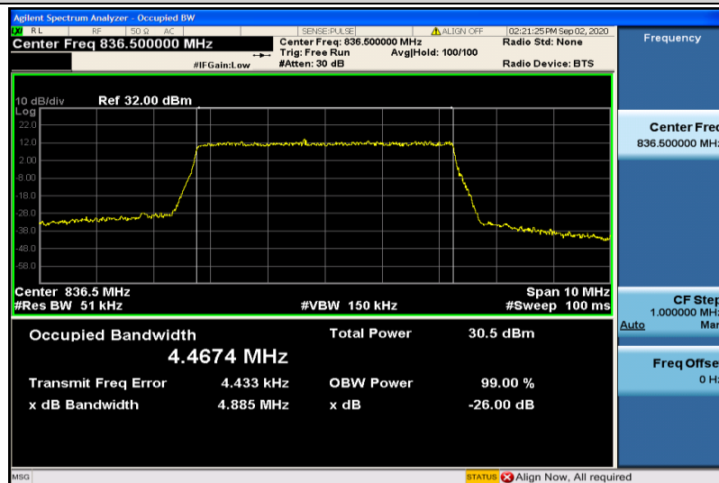
Band5-5MHz-QPSK-20525-25RB#0-4.4674
