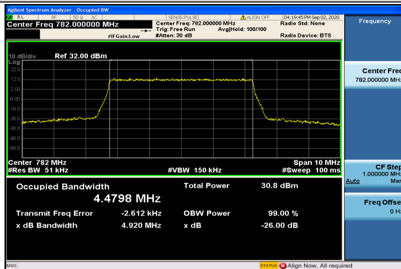
Band13-5MHz-QPSK-23230-25RB#0-4.4798
