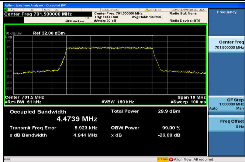
Band12-5MHz-16QAM-23035-25RB#0-4.4739
