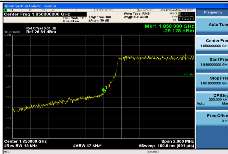
Band2-1.4MHz-QPSK-18607-6RB#0
