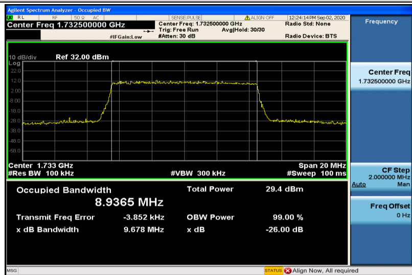
Band4-10MHz-16QAM-20175-50RB#0-8.9365
