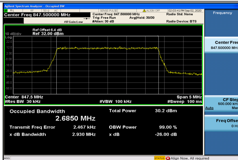
Band5-3MHz-QPSK-20635-15RB#0-2.6850
