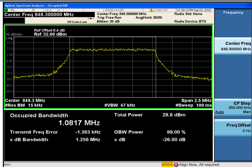
Band5-1.4MHz-16QAM-20643-6RB#0-1.0817
