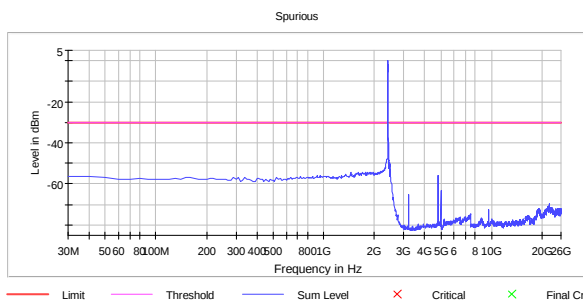
Conducted Emissions Ch01, 802.11n MCS8 MIMO
