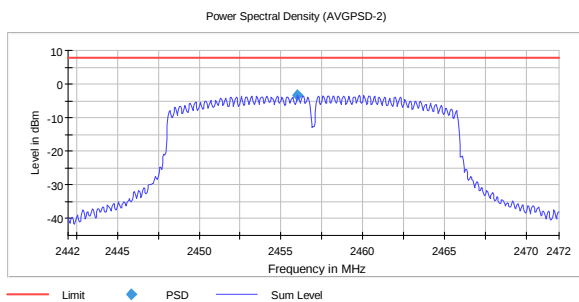
PSD, 2457 MHz, 802.11n MIMO MCS8 -3.29
