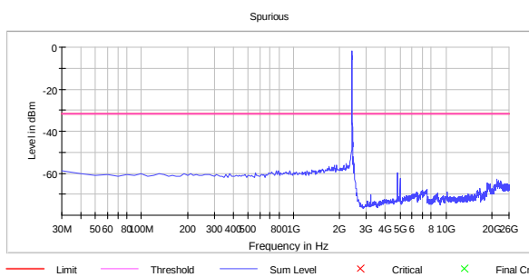
Conducted Emissions Ch01, 802.11n MCS0 SISO
