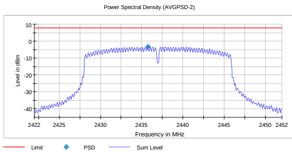
PSD, 2437 MHz, 802.11n MIMO MCS8 -3.24
