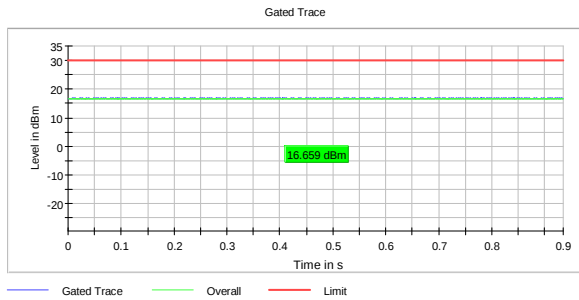
RMS Power, 2437 MHz, 802.11n MIMO MCS8
