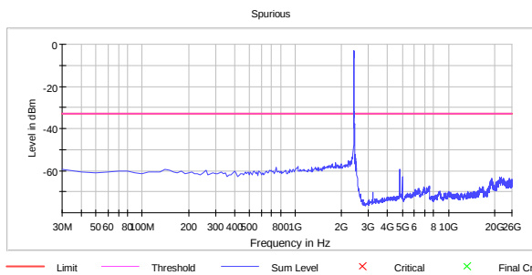
Conducted Emissions Ch01, 802.11g 6M
