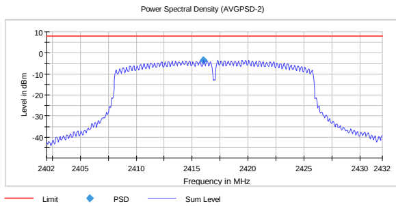
PSD, 2417 MHz, 802.11n MIMO MCS8 -3.55
