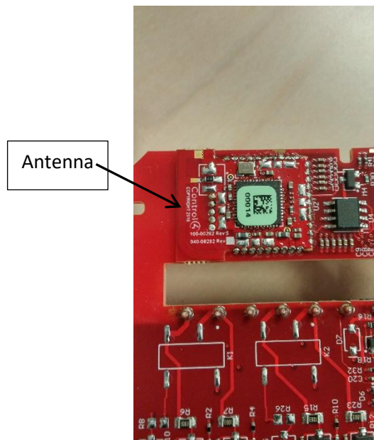
Photograph 5 – View of the RF Section of the EUT
