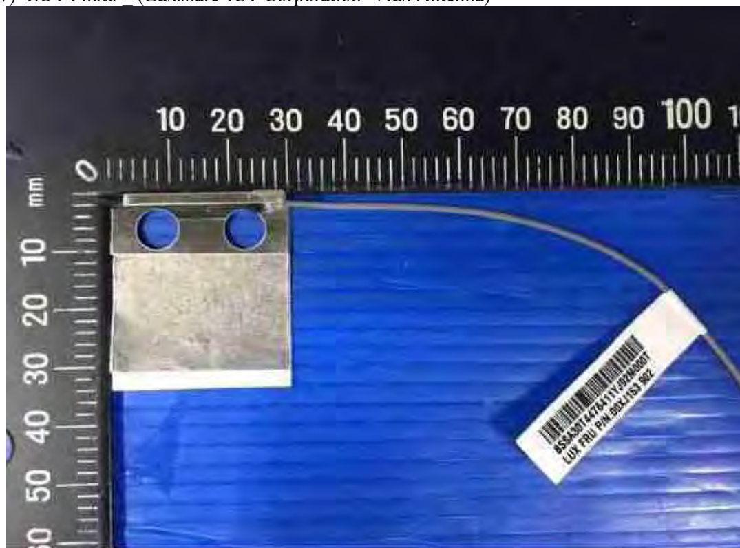
(28) EUT Photo
