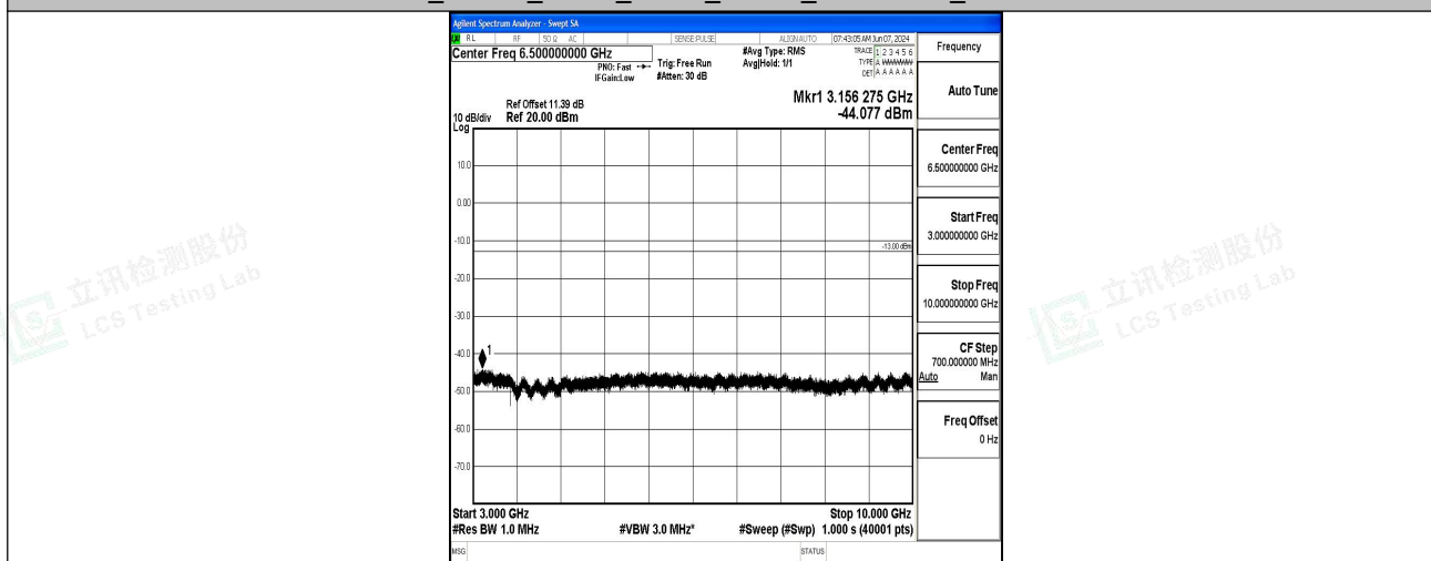
Band5_10MHz_QPSK_20525_1RB#0_3000~10000_3000~10000
