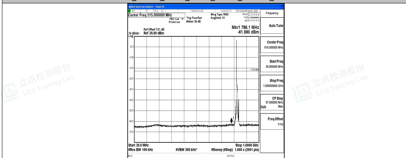
Band5_10MHz_QPSK_20450_1RB#0_30~1000_30~1000
