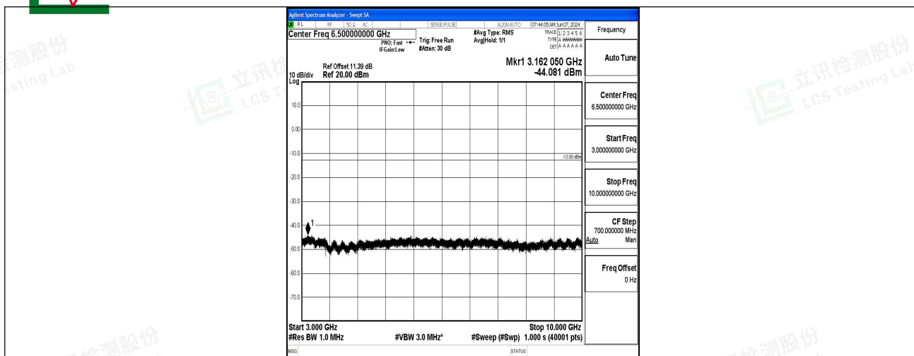
Band5_10MHz_QPSK_20600_1RB#0_3000~10000_3000~10000
