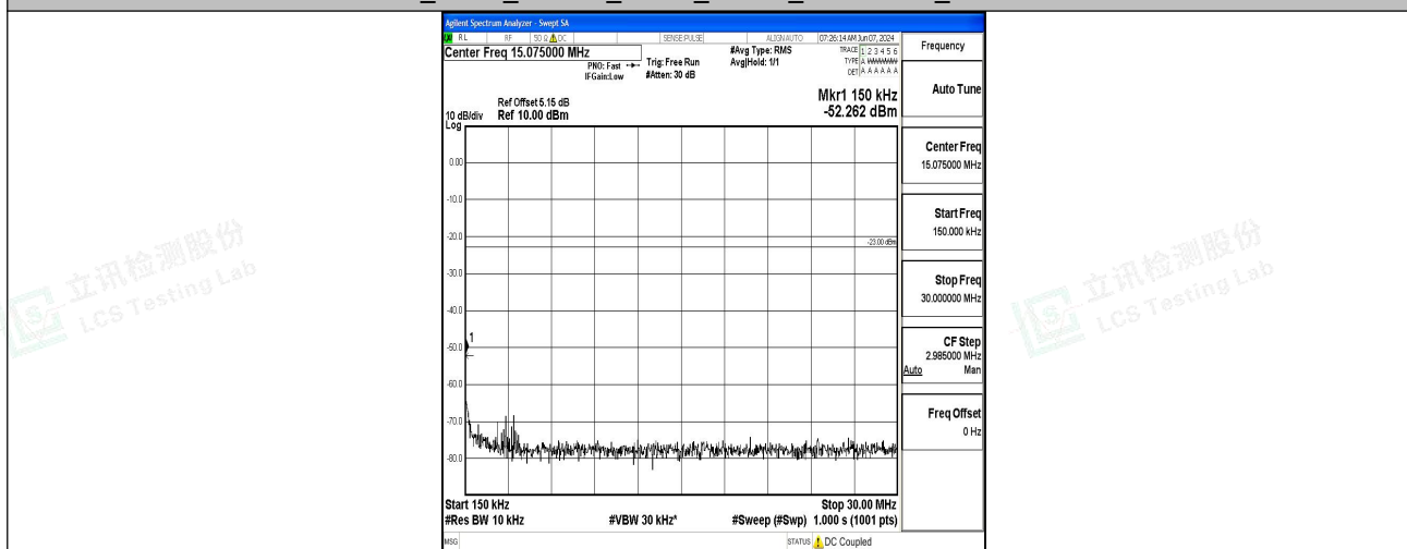
Band5_5MHz_16QAM_20625_1RB#0_0.15~30_0.15~30
