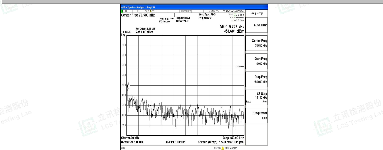
Band5_10MHz_QPSK_20525_1RB#0_0.009~0.15_0.009~0.15
