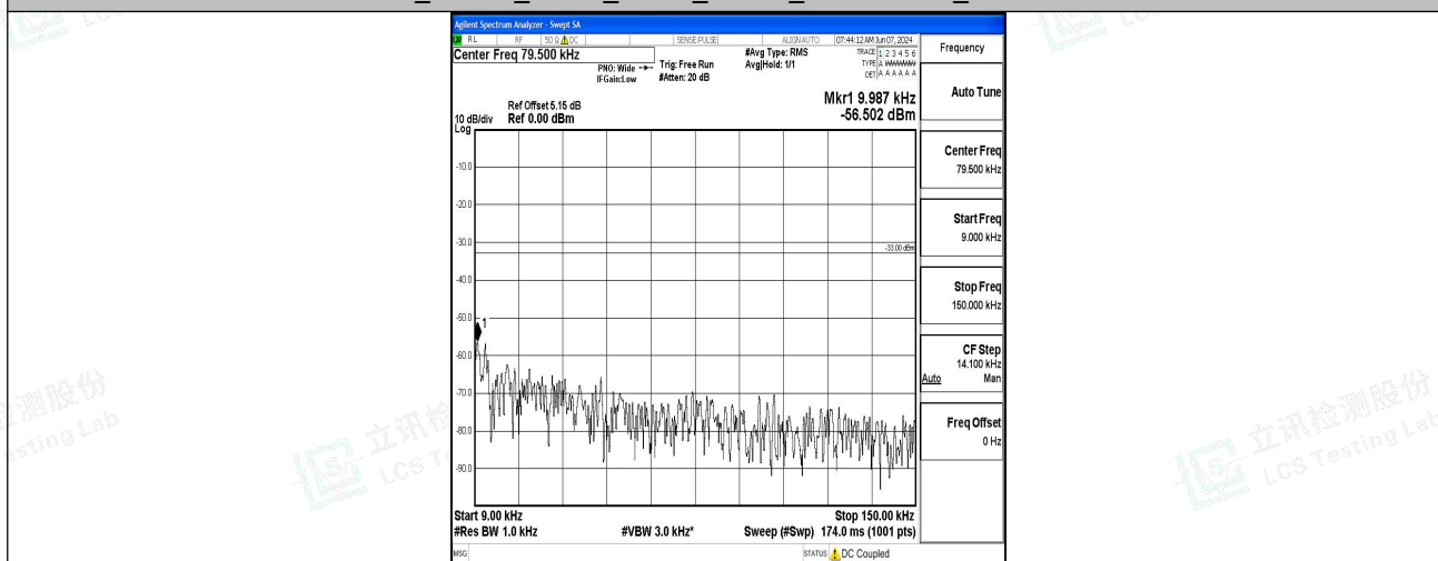
Band5_10MHz_16QAM_20600_1RB#0_0.009~0.15_0.009~0.15
