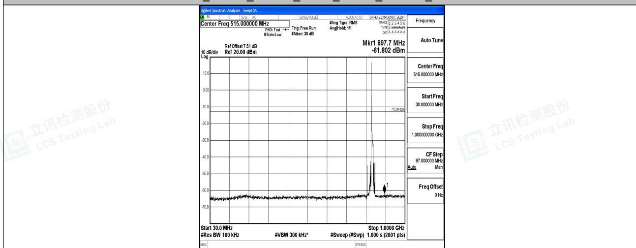
Band5_10MHz_16QAM_20525_1RB#0_30~1000_30~1000
