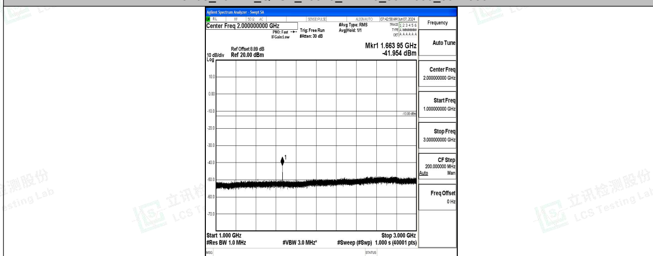
Band5_10MHz_QPSK_20525_1RB#0_1000~3000_1000~3000
