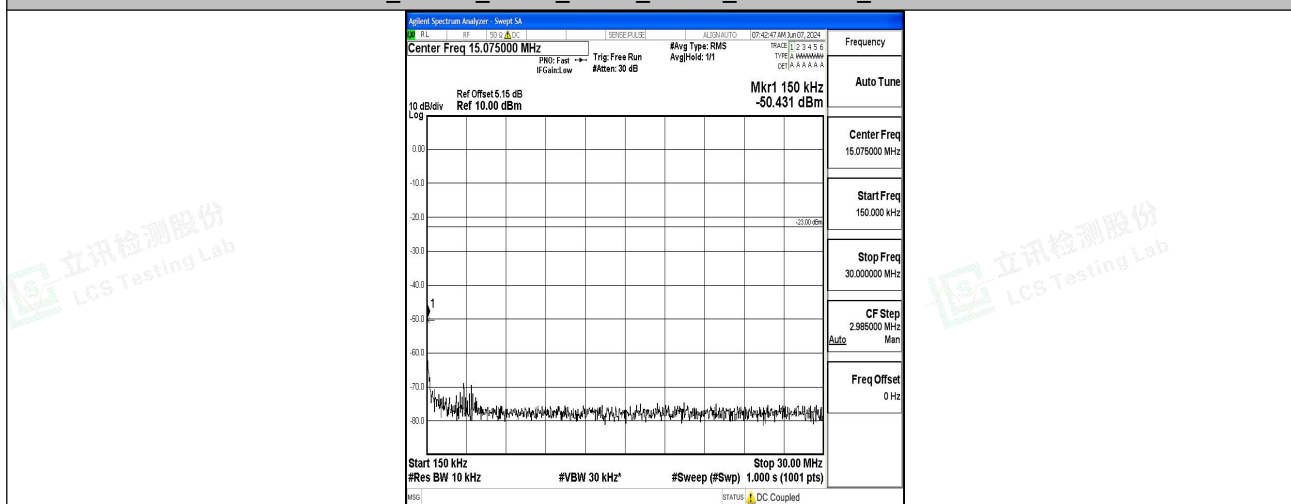
Band5_10MHz_QPSK_20525_1RB#0_0.15~30_0.15~30
