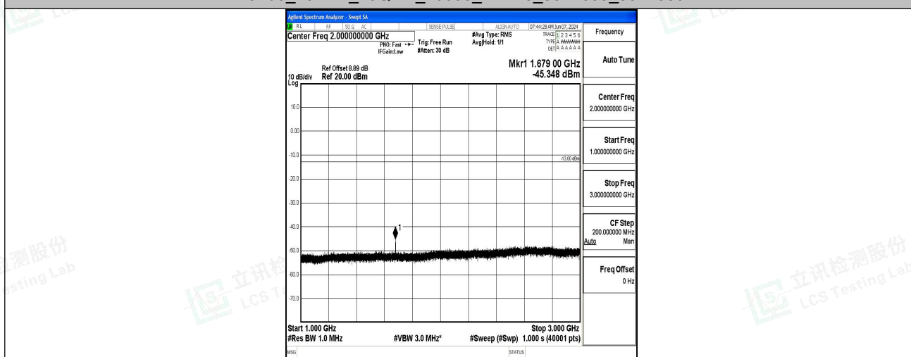
Band5_10MHz_16QAM_20600_1RB#0_1000~3000_1000~3000
