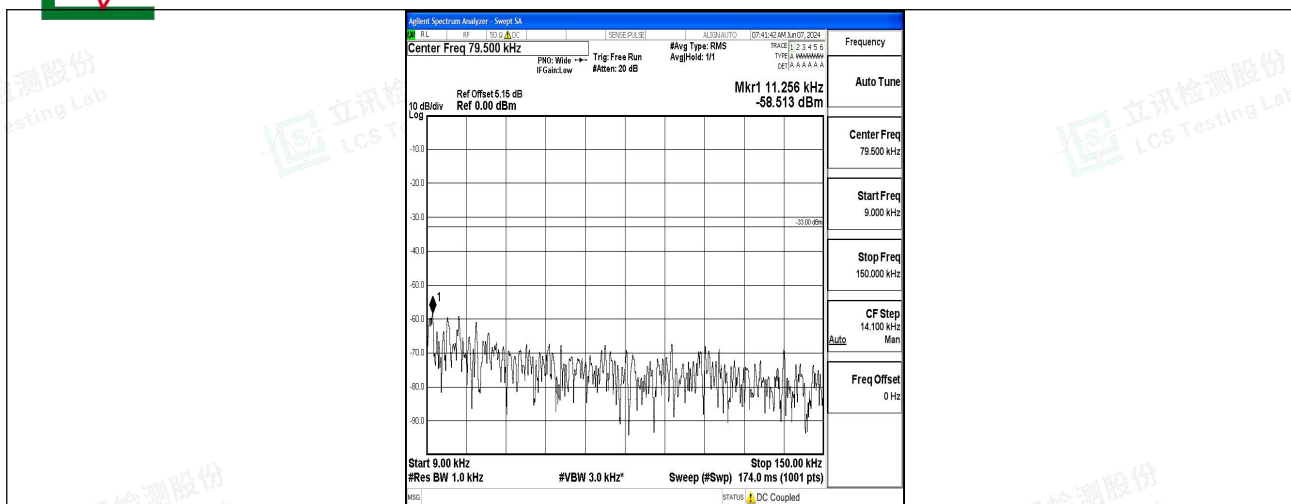
Band5_10MHz_QPSK_20450_1RB#0_0.009~0.15_0.009~0.15
