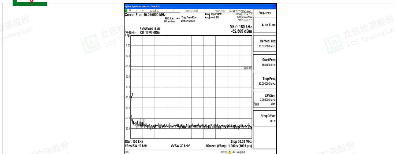
Band5_5MHz_QPSK_20625_1RB#0_0.15~30_0.15~30
