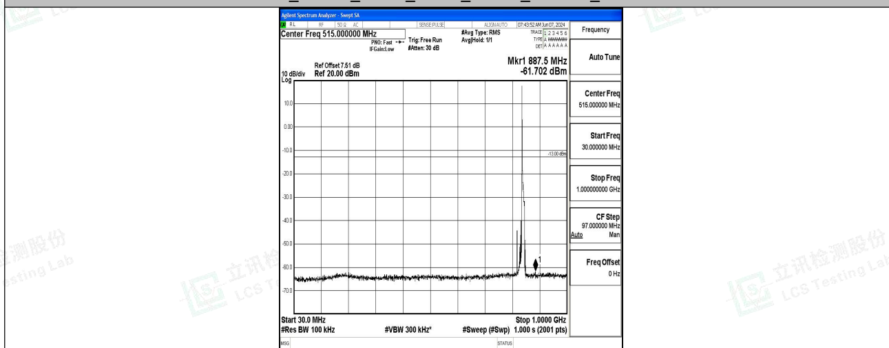
Band5_10MHz_QPSK_20600_1RB#0_30~1000_30~1000
