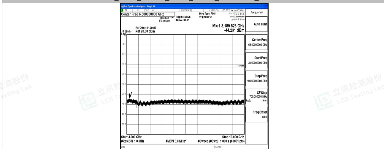
Band5_5MHz_16QAM_20525_1RB#0_3000~10000_3000~10000
