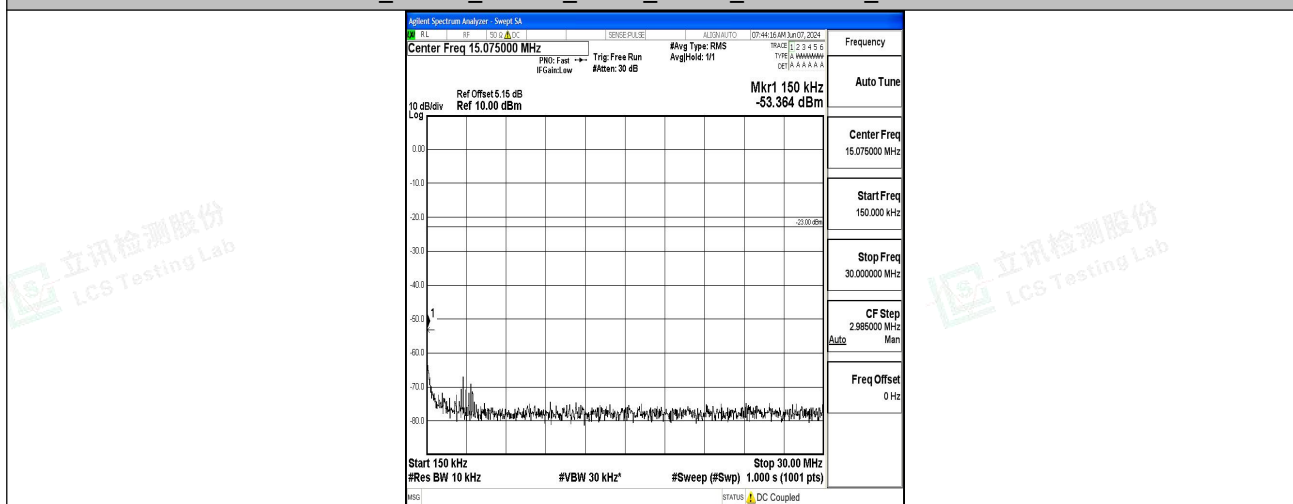
Band5_10MHz_16QAM_20600_1RB#0_0.15~30_0.15~30
