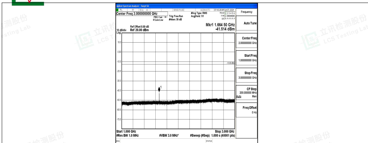
Band5_10MHz_16QAM_20525_1RB#0_1000~3000_1000~3000
