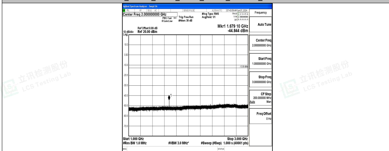
Band5_10MHz_QPSK_20600_1RB#0_1000~3000_1000~3000
