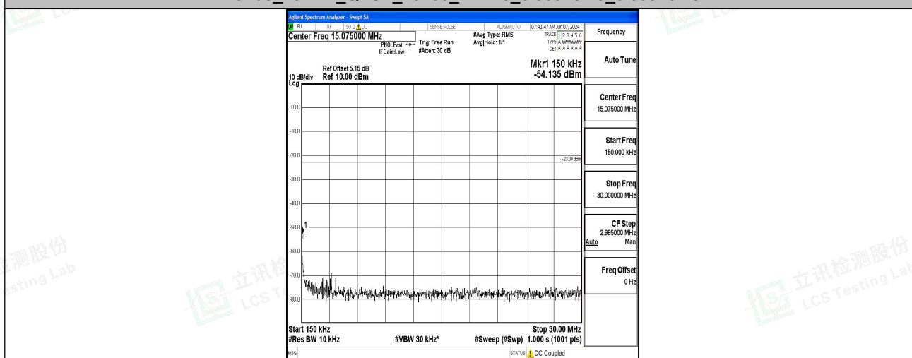
Band5_10MHz_QPSK_20450_1RB#0_0.15~30_0.15~30
