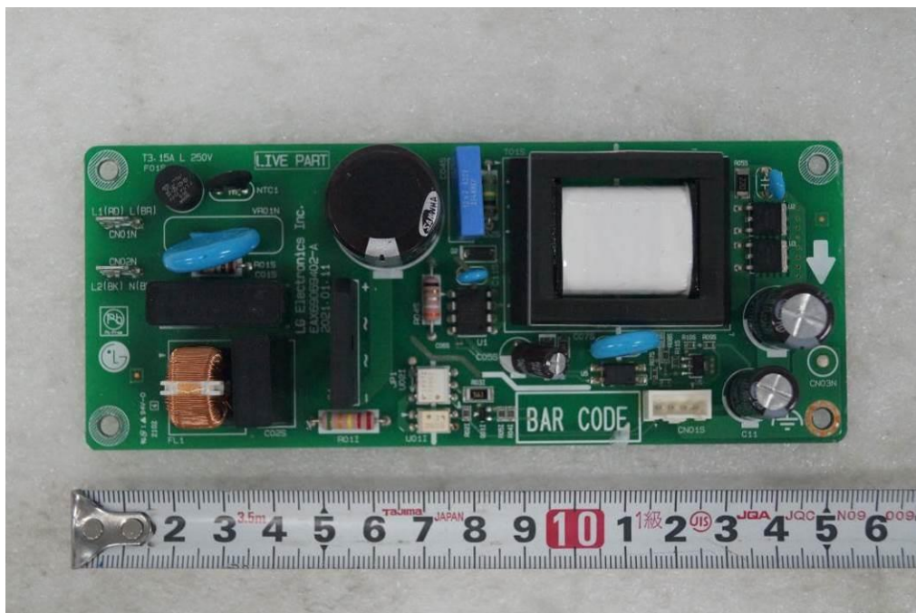
<OLD Power PCB>
