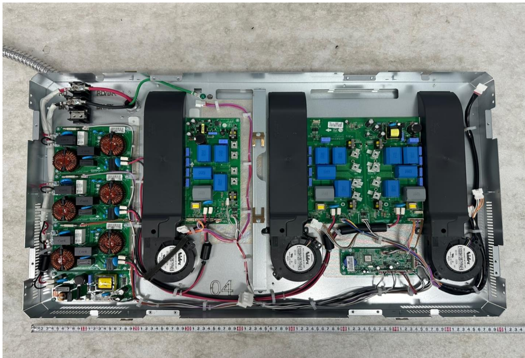
< New Inner of EUT >
