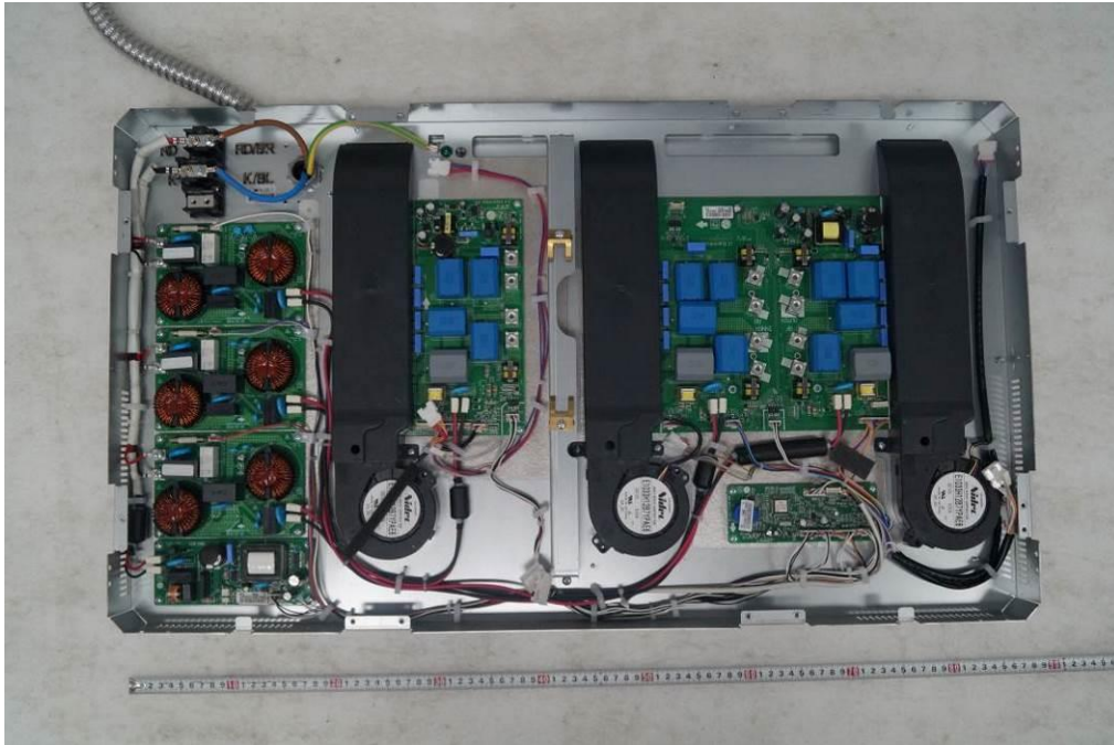
< OLD Inner of EUT >
