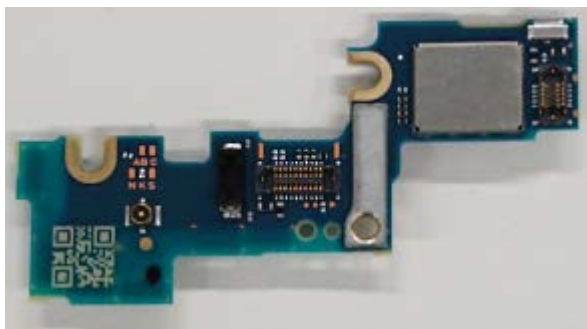
Internal Main_ANT-1-PWB (Front-side)
