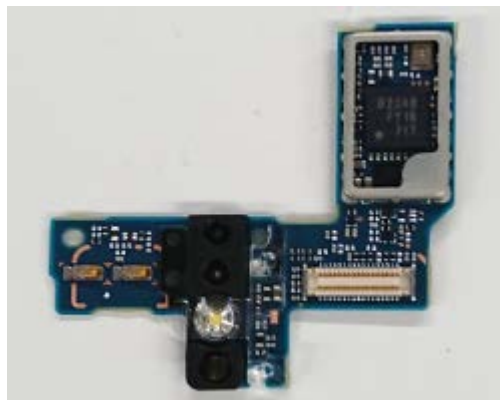
Internal Sub-PWB without Shield cases (Front-side)
