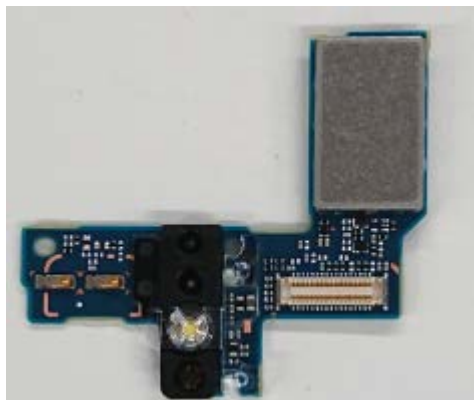
Internal Sub-PWB with Shield cases (Front-side)
