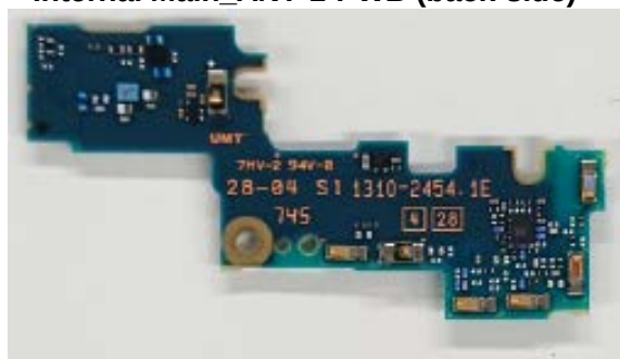
Internal Main_ANT-1-PWB (back-side)
