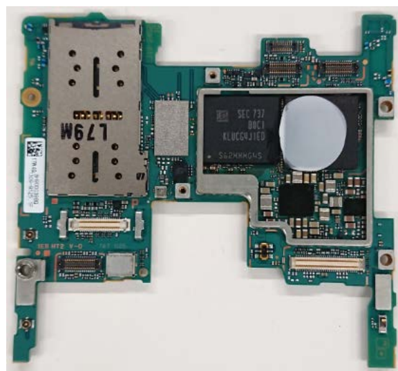
Internal PWB without Shield cases (Front-side)
