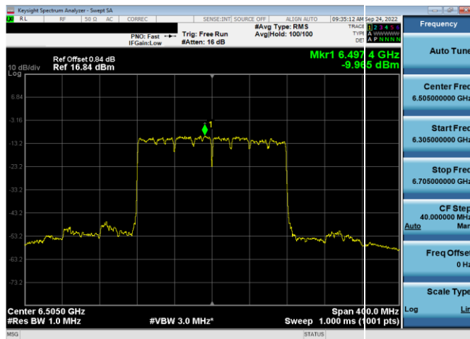
Plot 7-319. Power Spectral Density Plot SDM Antenna WF5t (160MHz 802.11ax (UNII Band 6) – Ch. 111, MCS11)
